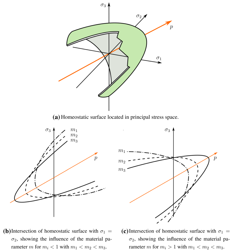
Fig. 2 Schematic representation of the homeostatic surface defined by Eq. (18) displayed in principal stress space. The hydrostatic axis p = \text{tr}(\mathbf{M} - \chi) is shown in orange. The eigenvalues of \mathbf{M} - \chi are denoted by \sigma_i
