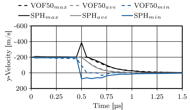
(b) Comparison of the maximum, minimum and average axial velocity in Ansys Fluent and SPH, the in-flight velocity of the droplet is directed in negative y -direction.
