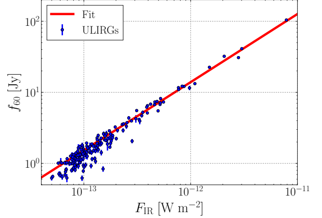
Figure 5. Correlation between the flux density at 60 \mu\text{m} , f_{60} , and the total IR flux between 8–1000 \mu\text{m} , F_{\text{IR}} , for our initial selection of 189 ULIRGs. The log-linear fit through these data points is also shown.
