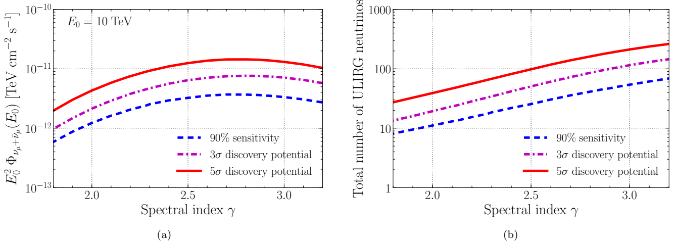
Figure 2. Sensitivity, 3 \sigma , and 5 \sigma discovery potentials as a function of the spectral index \gamma , for injected pseudo-signal following an unbroken E^{-\gamma} power-law spectrum. Panel (a) shows these quantities in terms of the flux at the normalization energy E_0 = 10 \text{ TeV} . Panel (b) shows them in terms of the mean number of injected pseudo-signal events. This number is found by convolving the injection spectrum with the effective area of the detector, and integrating it over energy and detector livetime.
