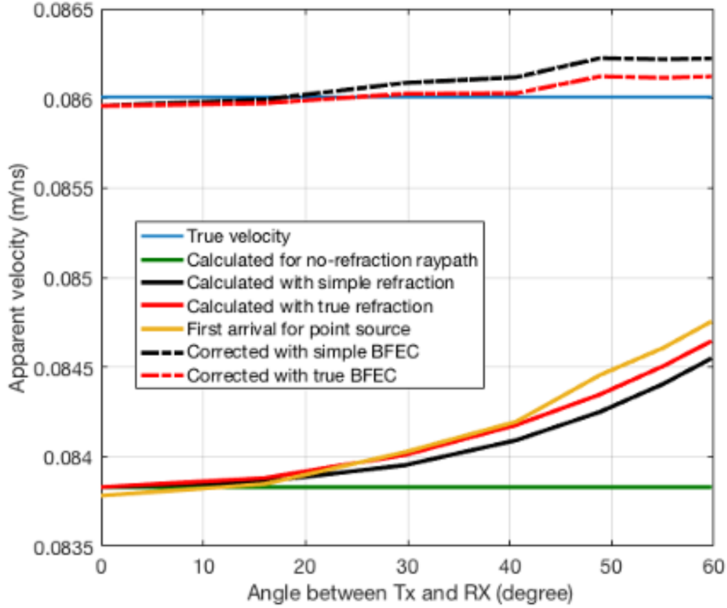
Figure 5.5: Average apparent-velocities of first arrival for point source (orange), assuming no refraction (green) and true velocity (blue) as shown in figure (5.3a) in the dashed rectangle. Calculated simple refraction apparent-velocities (black line) approach the first arrival values, whereas the true refraction apparent-velocities (red line) comes very close to first arrival values of the point source. Applying the simple BFEC and true BFEC returns apparent-velocities indicated by the dashed black and red lines, respectively, that approach the true velocity.
