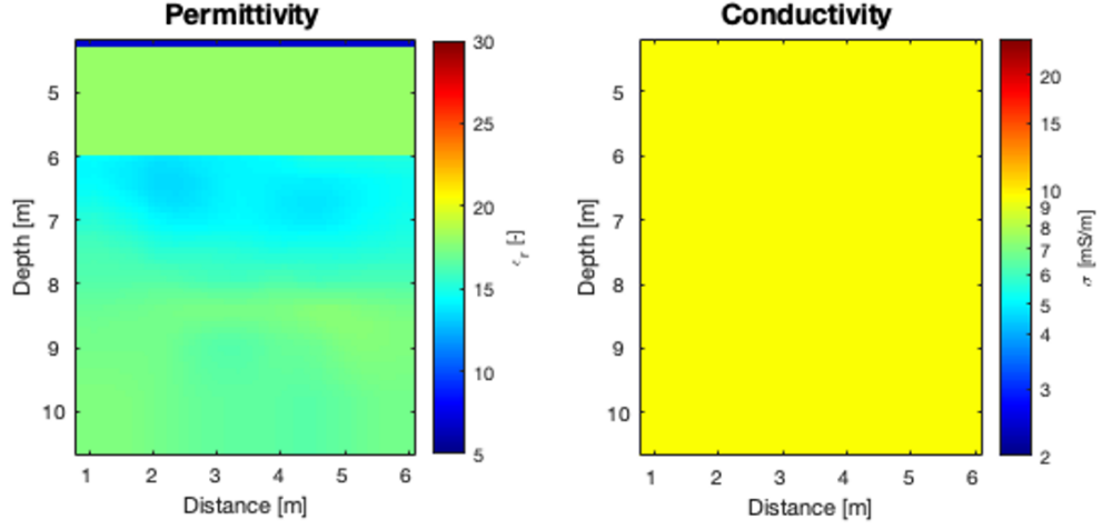
Figure 4.13: Left) \epsilon_r right) \sigma starting models that are used for 2D, 2.5D vanilla and borehole-integrated FWI
