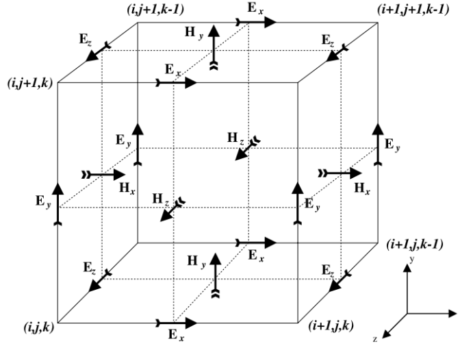
Figure 2.2: The Yee cell adopted from Giannopoulos [52].
