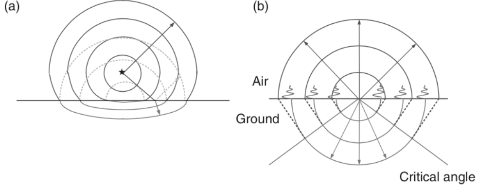
Figure 2.1: Wavefronts spreading out from a localised source. In (a), the source is located above the ground. The dotted lines indicate the reflected signal. In (b), the source is located on the air-ground interface. The dashed lines indicate refracted waves. The oscillating lines indicate evanescent waves, adopted from Annan [4].
