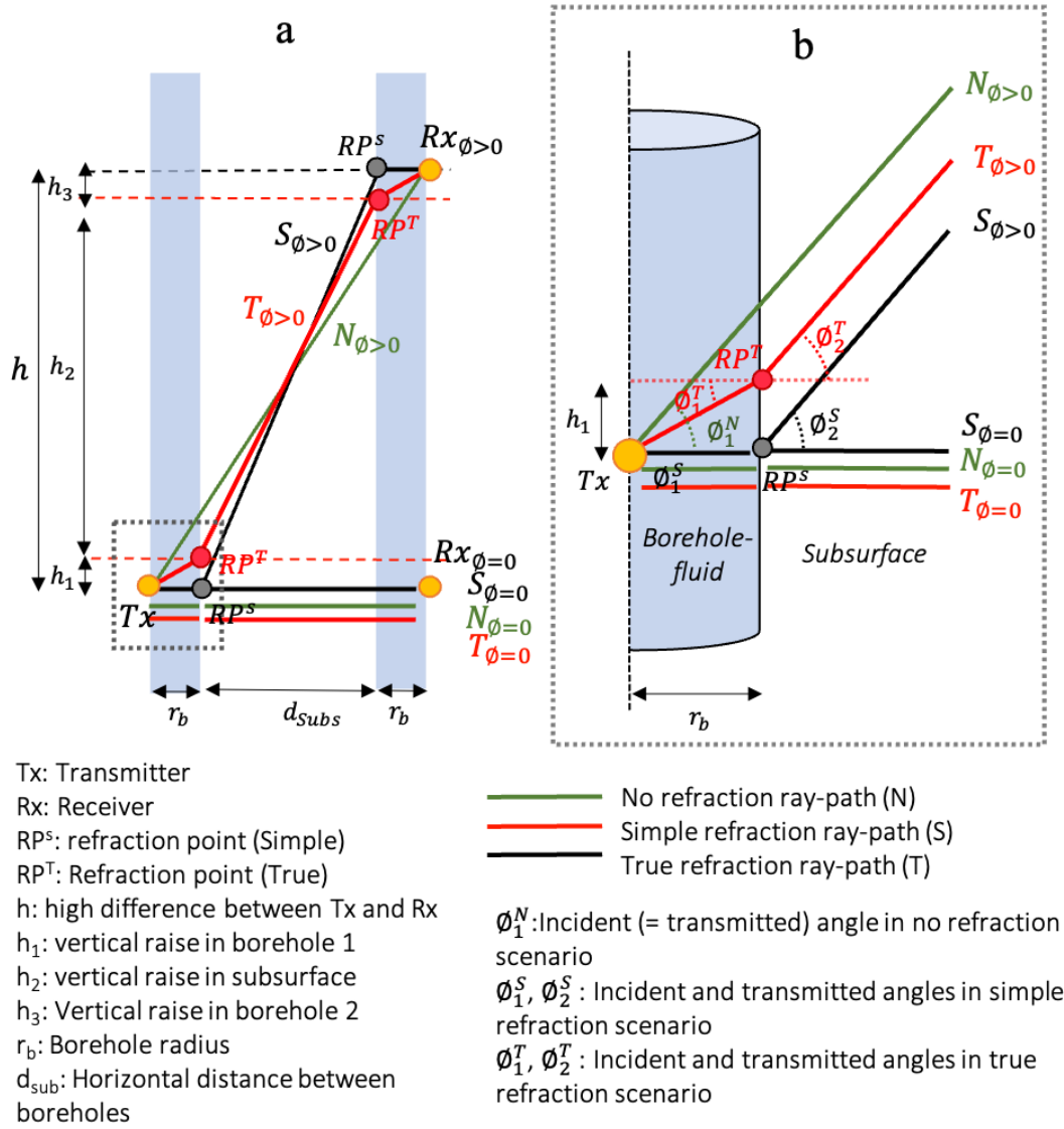
Figure 5.2: a) Ray paths with no refraction (N), true refraction (T), and simple refraction (S) for zero-degree ( \phi = 0 ) and arbitrary ( \phi > 0 ) ray angle b) Close up view of the ray-paths at the interface between the borehole-fluid and the subsurface where the refraction point for simple refraction and true refraction are indicated by ( RP^S ) and ( RP^T ), respectively.
