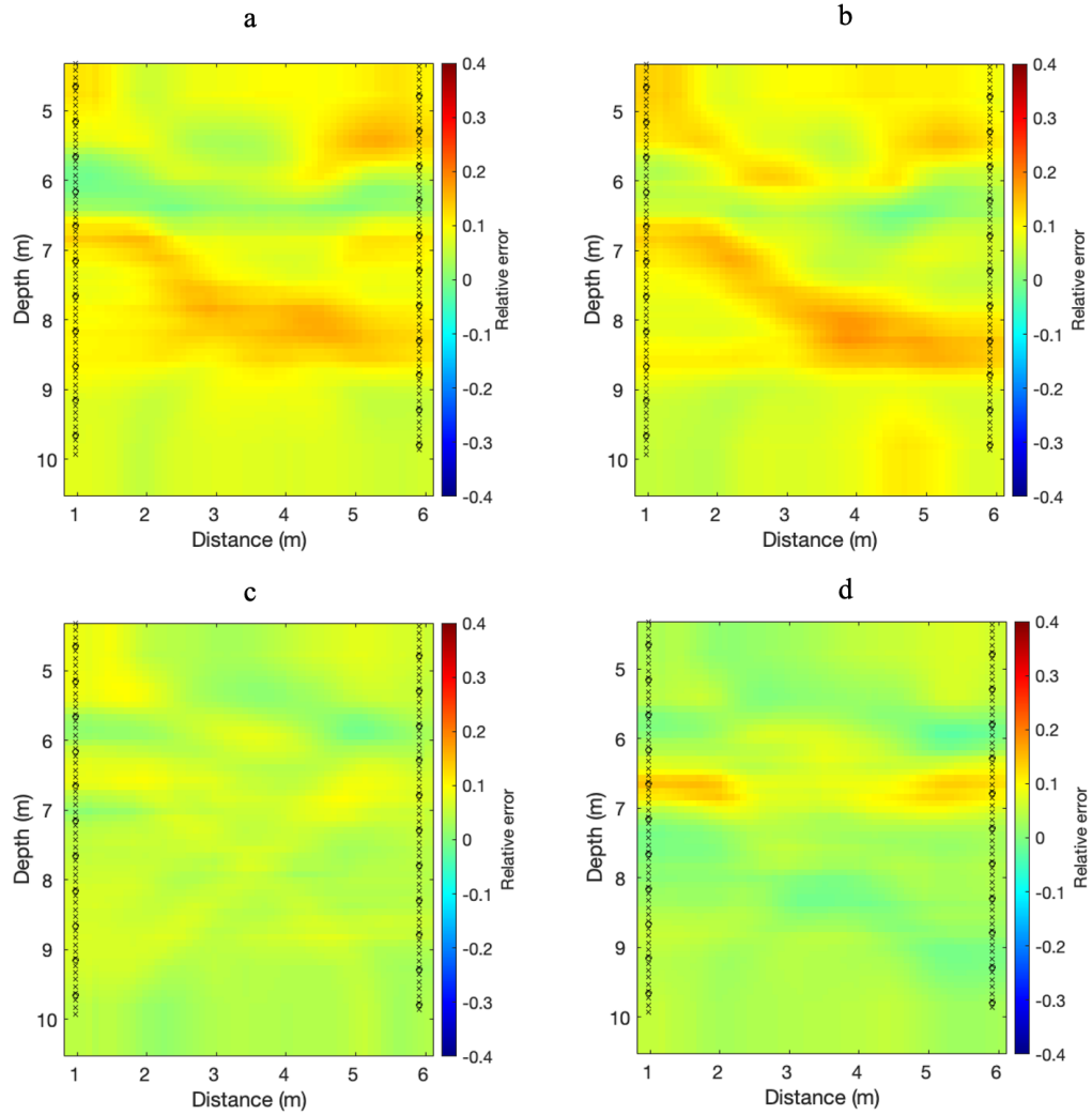
Figure 5.10: Relative difference in estimated \epsilon_r of no borehole case in compare to a) traveltime inversion without BFEC b) traveltime inversion with limited angular aperture and without BFEC c) traveltime inversion with simple BFEC and d) traveltime inversion with true BFEC. Tx and Rx positions are indicated by circles and crosses, respectively.
