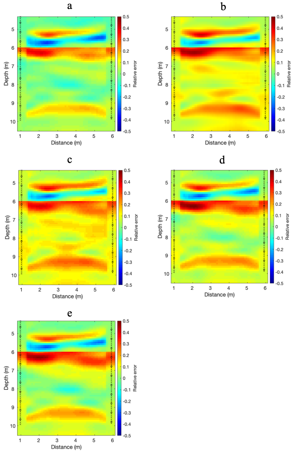
Figure 5.8: Relative model error in estimated \varepsilon_r for traveltime inversions for a) no borehole present, b) t water-filled borehole without BFEC c) water-filled borehole without BFEC, and limited aperture, d) water-filled borehole with simple BFEC, and e) water-filled borehole with BFEC. Tx and Rx positions are indicated by circles and crosses, respectively.
