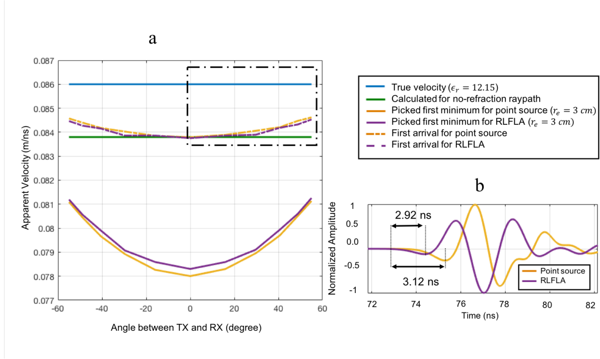
Figure 5.3: a) Average apparent-velocities obtained from picked first minimums for point source (orange) and RLFLA (purple) antennas. The first arrival traveltimes for point source and the first arrival traveltimes with compensation for antenna thickness for RLFLA are indicated by the orange and purple dashed lines, respectively. Calculated apparent-velocities for raypaths without refraction are shown by the green line, whereas the true velocity of the medium is indicated by the blue line. b) Picked first minimum for point source and RLFLA and compensation for antenna-thickness that causes an earlier arrival for RLFLA due to the lower \epsilon_r of the antenna insulation than borehole-fluid.
