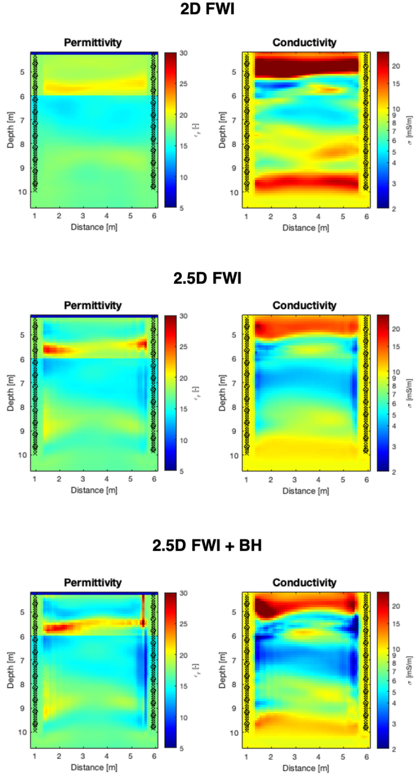
Figure 4.16: Left) \epsilon_r and right) \sigma models for 2D (above), 2.5D FWI (middle), 2.5D FWI with borehole-fluid integration (bottom) Note the logarithmic scale for \sigma tomograms. Tx and Rx positions are indicated by circle and crosses, respectively.
