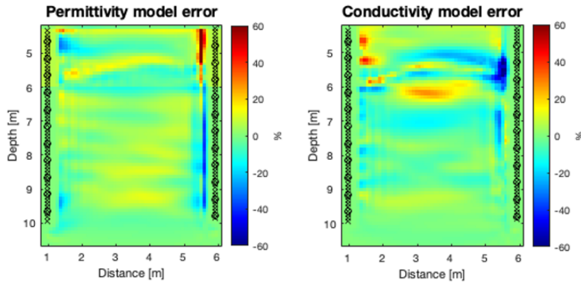
Figure 4.17: Left) model error percentage of \epsilon_r and right) of \sigma models for 2D (above), 2.5D FWI (middle), 2.5D FWI with borehole-fluid integration (bottom). Transmitter and receiver positions are indicated by circle and crosses, respectively.
