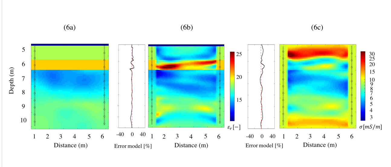
Figure 3.6: \varepsilon_r and \sigma Updated \varepsilon_r starting model (a), \varepsilon_r (b) and \sigma (c) resulting tomograms of the 2.5D FWI and the corresponding lateral average model errors on the left side. Note the logarithmic scale for \sigma tomogram. Tx and Rx positions are indicated by circle and crosses, respectively.
