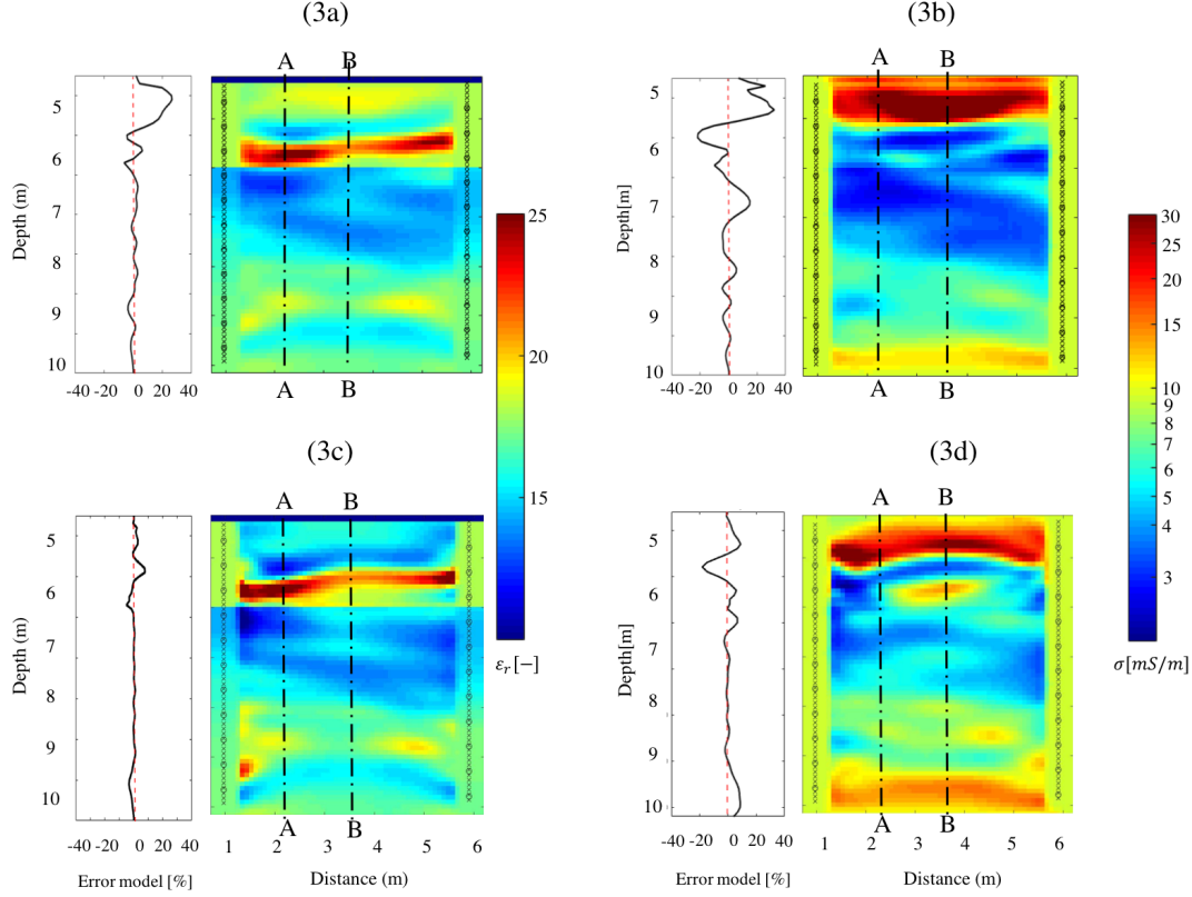
Figure 3.3: The (a),(c) are \varepsilon_r models and are (b),(d) \sigma models for 2D and 2.5D FWI respectively, while corresponding lateral average errors plotted on the left side of the tomograms. A-A and B-B show the positions of the cross-sections presented in figure (3.4). Note the logarithmic scale for \sigma tomograms. Tx and Rx positions are indicated by circle and crosses, respectively.
