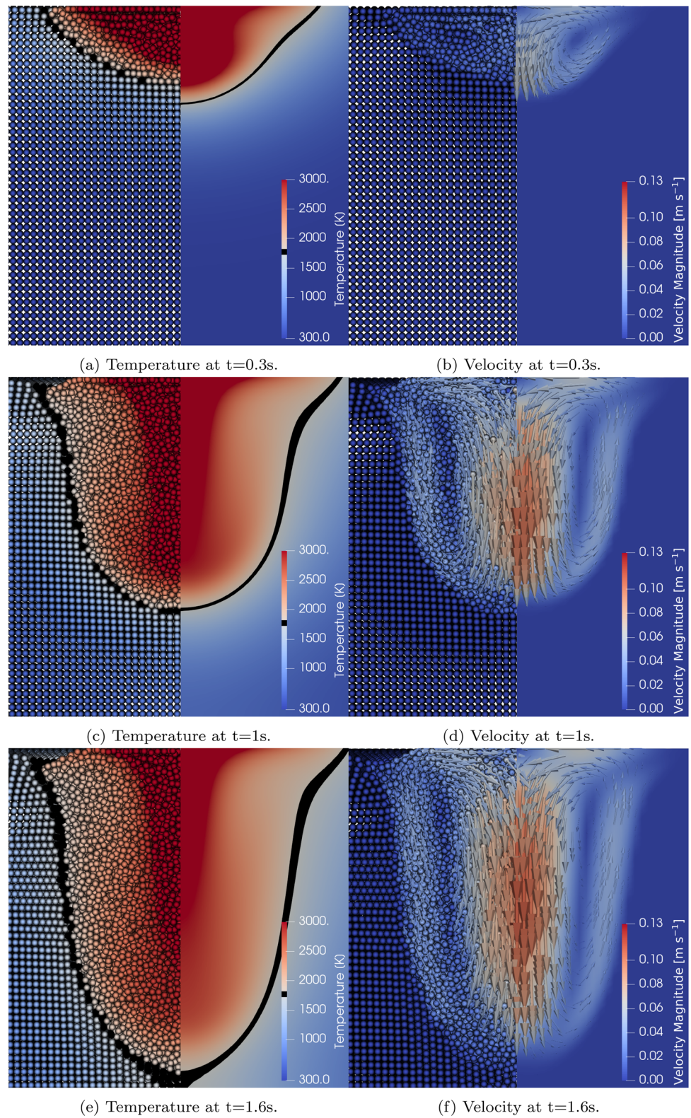
Fig. 14 Side-by-by comparison of SPH and FEM results of temperature (left column) and velocity (right column). The SPH solution is always shown on the left within each figure, while the WM solution is shown on the right
