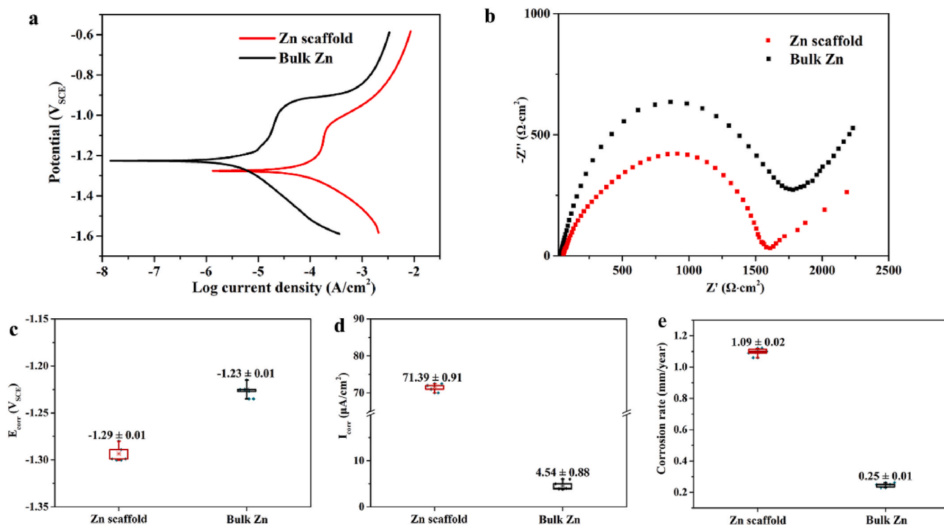
Fig. 2. Electrochemical test of pure Zn porous scaffold and dense pure Zn in Hanks' solution: (a) Potentiodynamic polarization curve; (b) Nyquist plot; (c) Corrosion potential ( E_{\text{corr}} ); (d) Corrosion current density ( I_{\text{corr}} ); (e) Corrosion rate.
