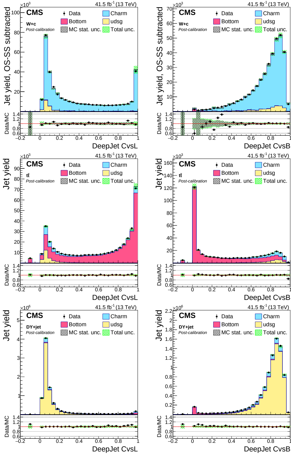
Figure 18: Post-calibration DeepJet CvsL (left) and CvsB (right) distributions of jet samples selected from W+c (upper), t\bar{t} semi- and dileptonic (middle), and DY + \text{jet} (lower) events after application of DeepJet c tagger shape calibration SFs. The bin corresponding to a tagger value of -1 is plotted at -0.1 . Vertical error bars in data represent statistical uncertainties in data. The simulations are shown as stacked histograms.
