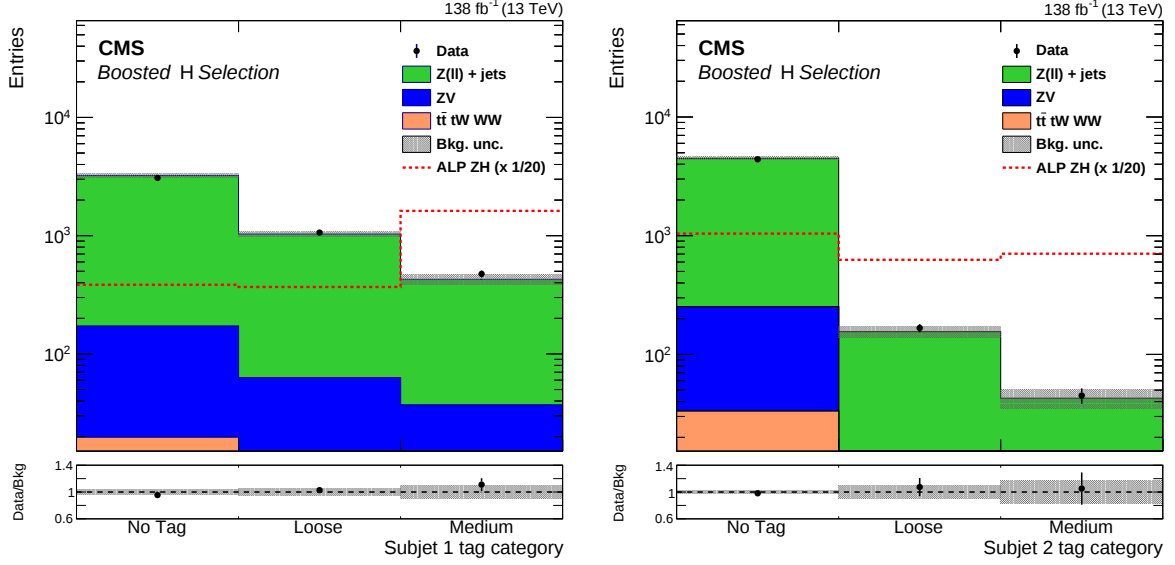
Figure 3: Distributions of the untagged, exclusive loose, and medium DEEPCSV tags for the more b-like subset (left) and the less b-like subset (right) of the boosted hadronic H candidates in SR2. The gray band shows the statistical and systematic uncertainties in the background. Background normalizations are derived from the final fit to the data. The red dashed histograms correspond to a hypothetical chiral ALP with 1 \text{ TeV}^{-1} couplings to gluons and ZH, and f_a = 3 \text{ TeV} ; the cross sections have been multiplied by the factors indicated in the legends for better visibility. The lower panels show the ratio of data to background.
