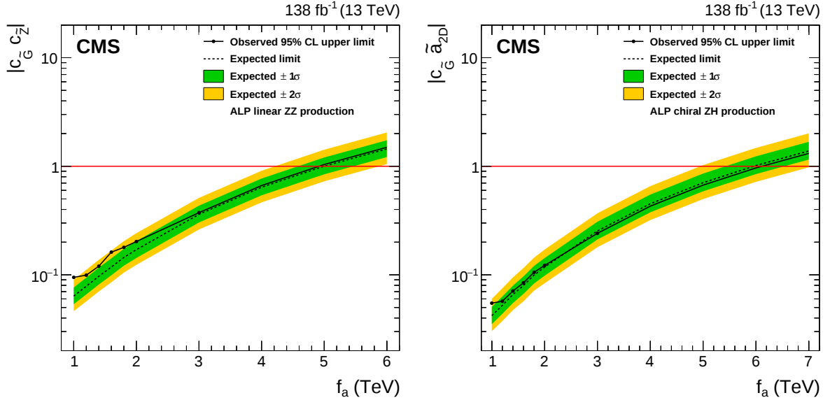
Figure 9: Observed and expected 95% CL upper limits on the ALP linear |c_{\tilde{G}} c_{\tilde{Z}}| (left) and the ALP chiral |c_{\tilde{G}} \tilde{a}_{2D}| (right) coupling coefficients as a function of the mass scale f_a for ALP masses m_a < 100 GeV.
