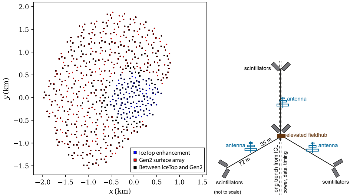
Figure 1: Layout of the IceCube-Gen2 Surface Array (left) and station design (right). The layout builds on the IceTop enhancement using the same station design of 4 pairs of scintillators and 3 surface radio antennas connected to a local DAQ in an elevated fieldhub. There will be one station on top of each string of the Gen2 optical array in addition to a few stations filling gaps to the planned surface enhancement of IceTop.
