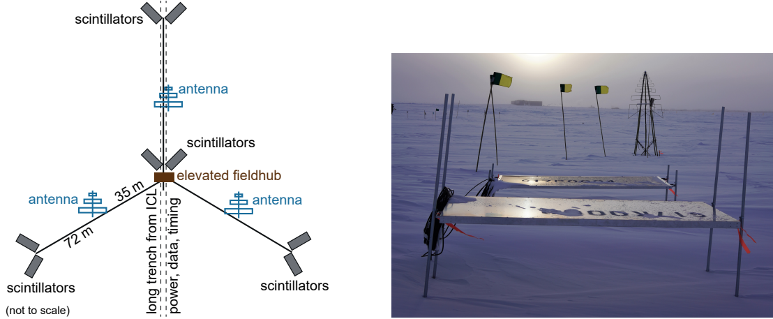
Figure 3: (Left) Layout of a surface station for the enhancement of IceTop, which is also the baseline design for the Gen2 surface array. (Right) Corresponding prototype detectors at IceTop; both the scintillators and radio antennas are deployed on stands that can be lifted to avoid snow management.
