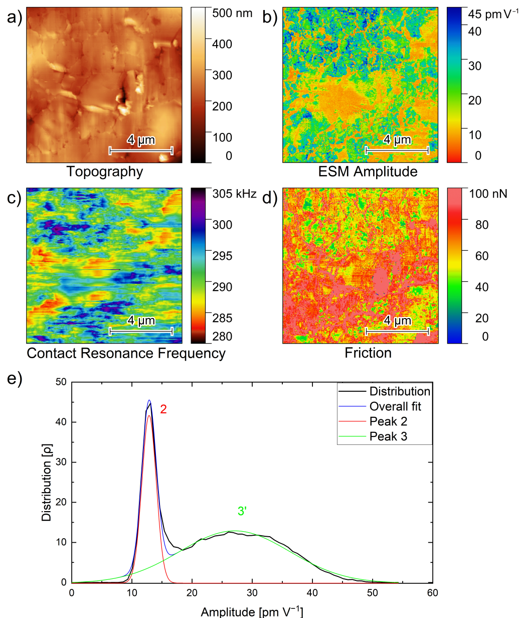
Figure 4. (a) Topography, (b) amplitude, (c) contact resonance frequency, (d) friction images and (e) amplitude distribution graph of Figure 4b, of a 10 μm × 10 μm area of a PEO 6 –LiTFSI film with 50 wt.% LLZO:Ta film polished with a focused ion beam. Peak 3' reflects the overlapping peaks 3 and 4.
