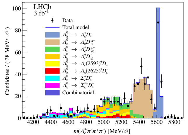
FIG. 3. Distribution of the \Lambda_c^+ \pi^- \pi^+ \pi^- invariant mass for the \Lambda_b^0 \rightarrow \Lambda_c^+ D_s^-(X) control sample, with D_s^- \rightarrow \pi^- \pi^+ \pi^- . The components contributing to the fit model are indicated in the legend.
