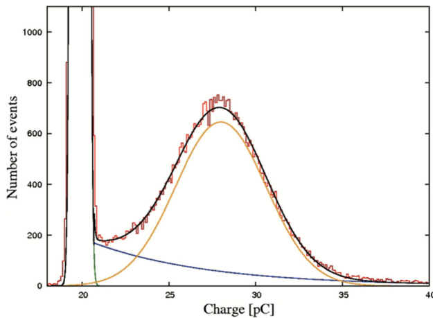
Fig. 20 Typical single photoelectron charge response [38]. Pedestal and SPE peaks are fit by two gaussians, adding an exponential to describe the valley region
