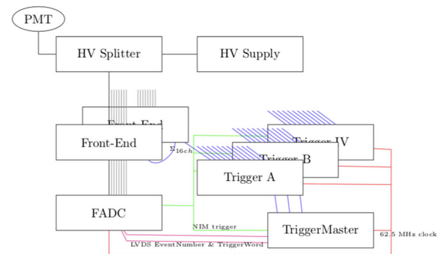
Fig. 22 Double Chooz simplified electronics scheme
