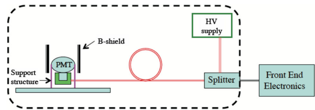
Fig. 11 Schematic of Inner PMT system
