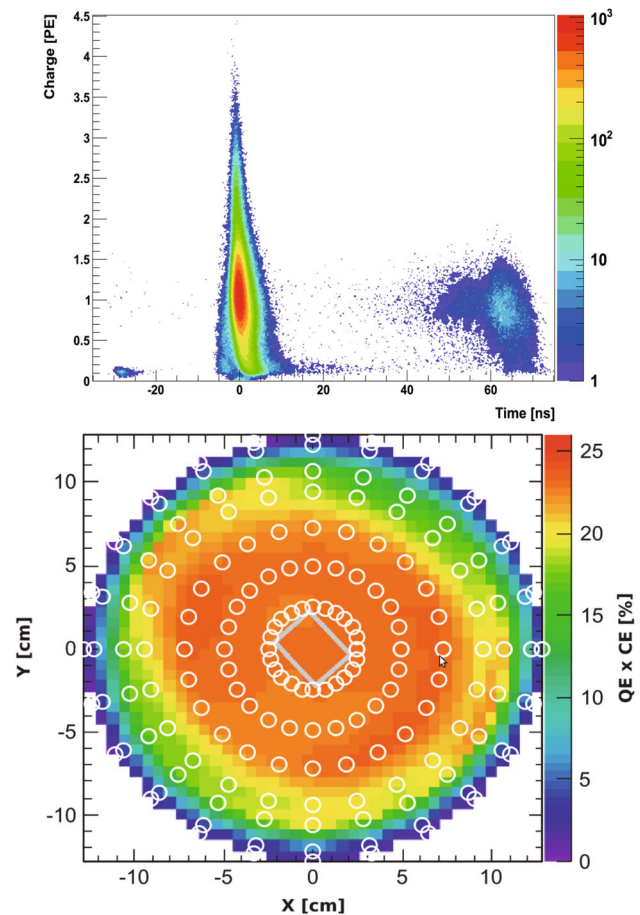
Fig. 21 Transit time versus charge plotted event by event [39] (top). One can identify main pulses around t = 0 ns with a transit time spread of \approx 3 ns, pre-pulses around t = -25 ns and late-pulses up to t = 70 ns. The fraction of single PE in the measured population was about 95%
