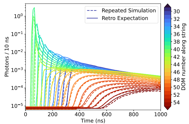
Fig. 7 Expected photon time distribution in several DOMs along string 86, for a straight up-going muon with an energy 20 GeV, starting at (0, 0, -350)\text{ m} in IceCube coordinates. The dashed lines show the average from 10^7 repeated MC simulations, while the solid lines show the expected distributions based on the tables and event model discussed here
