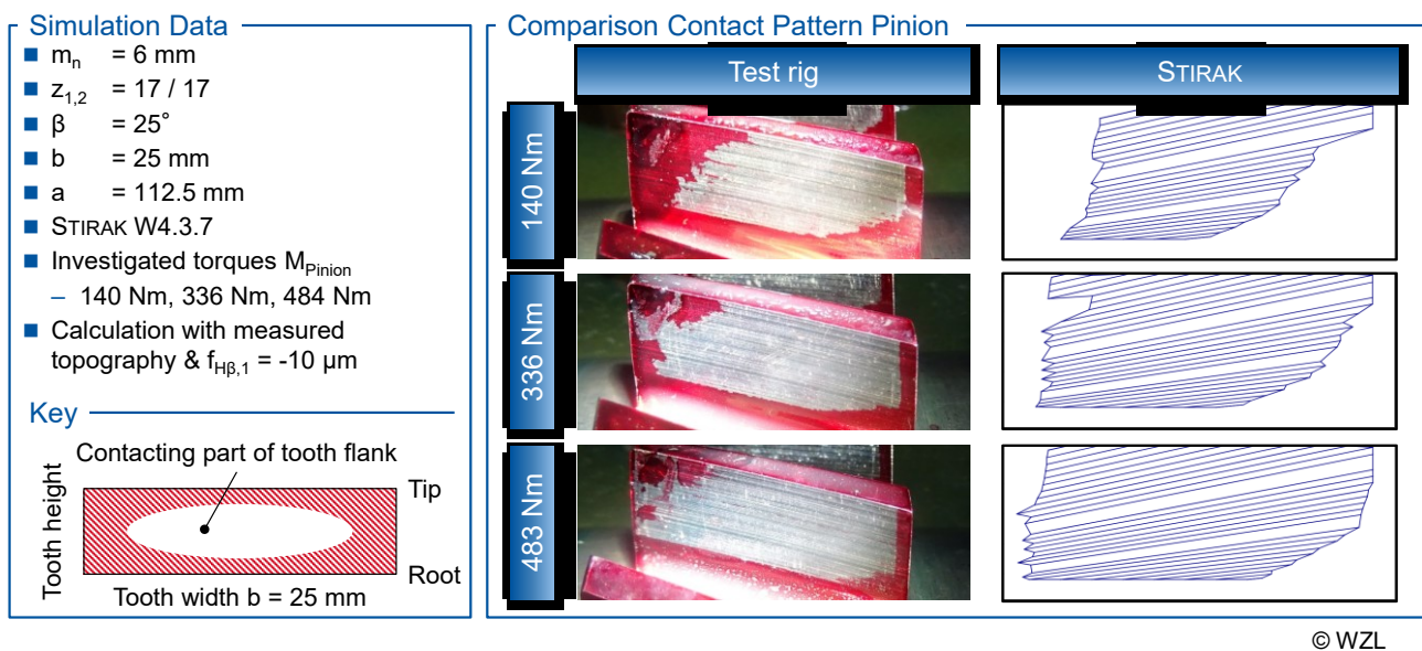
Figure 5-2: Comparison of contact patterns
