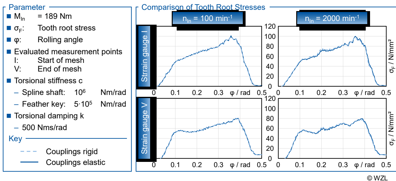
Figure 5-3: Impact of stiffness on the calculated tooth root stress
