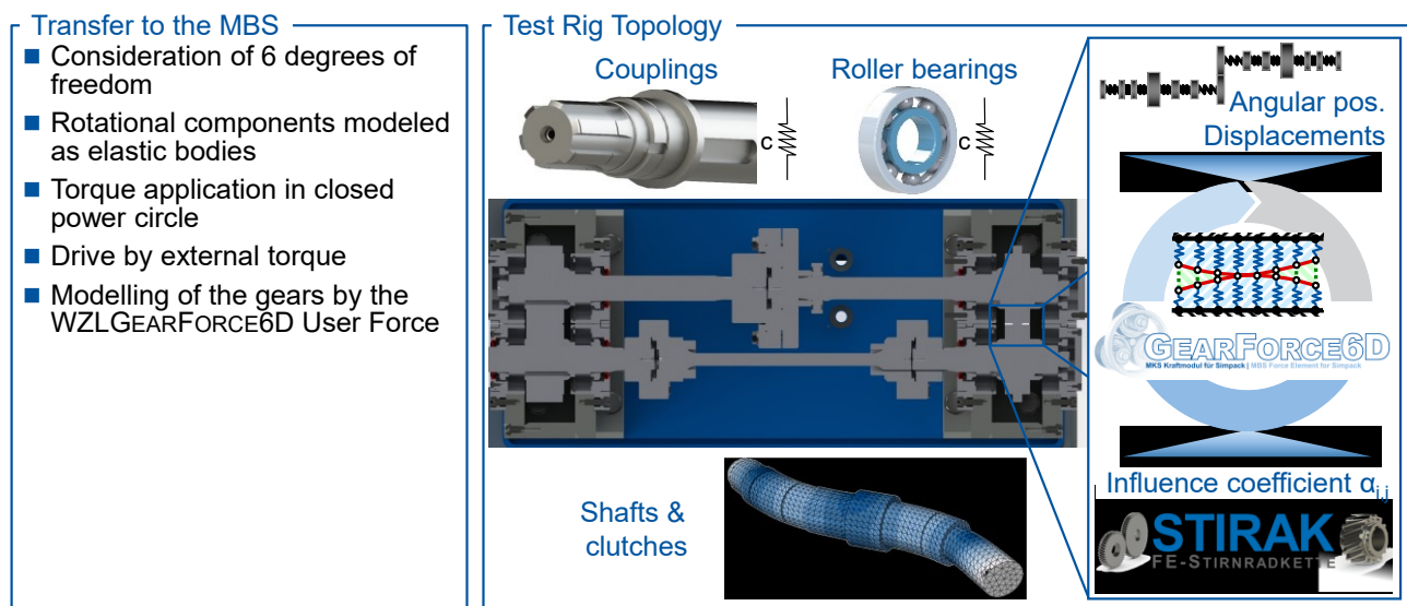
Figure 5-1: Transfer of the test rig to the multi body simulation
