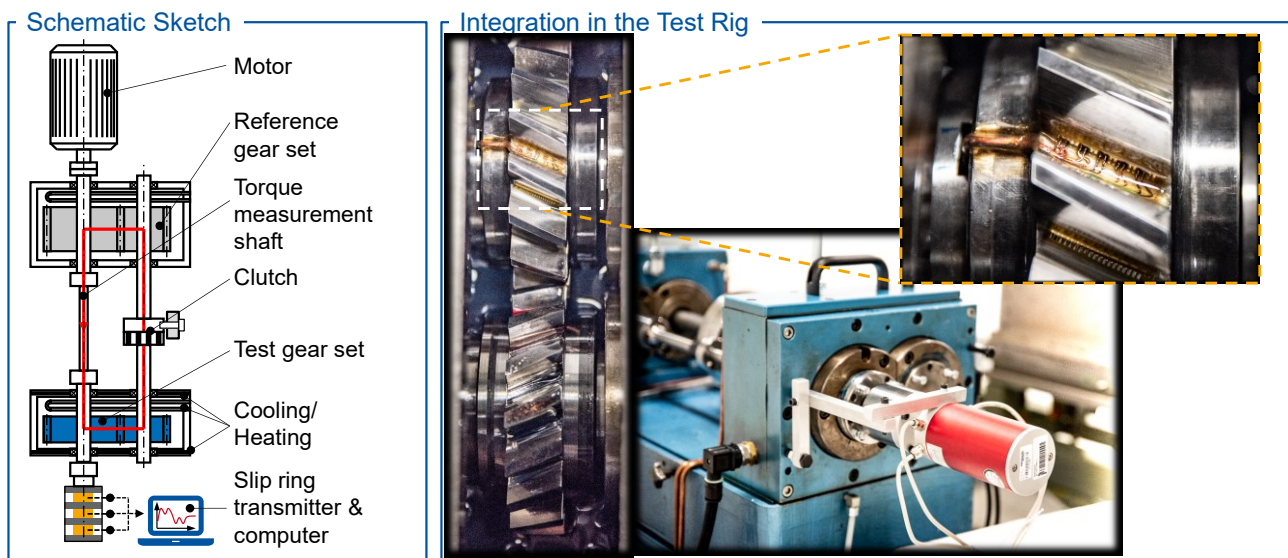
Figure 4-2: Test rig setup for the measurement of the tooth root strain
