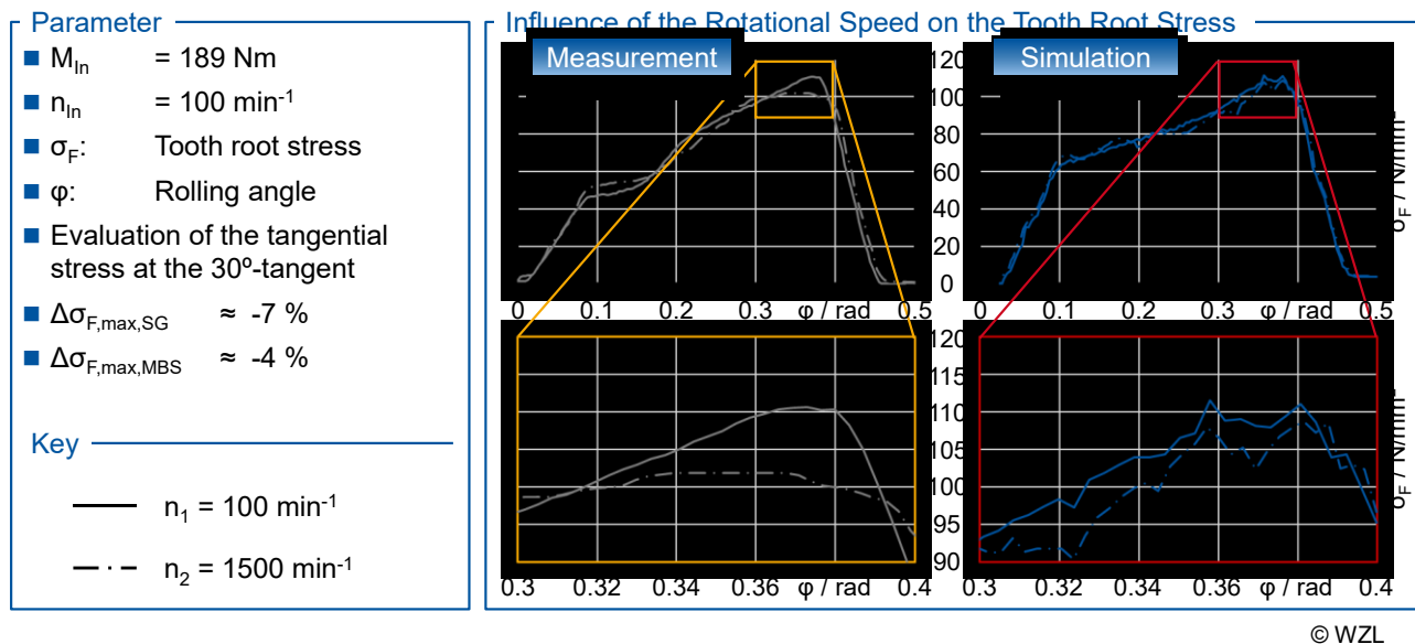
Figure 6-2: Comparison of calculated and measured tooth root stress at variable speeds
