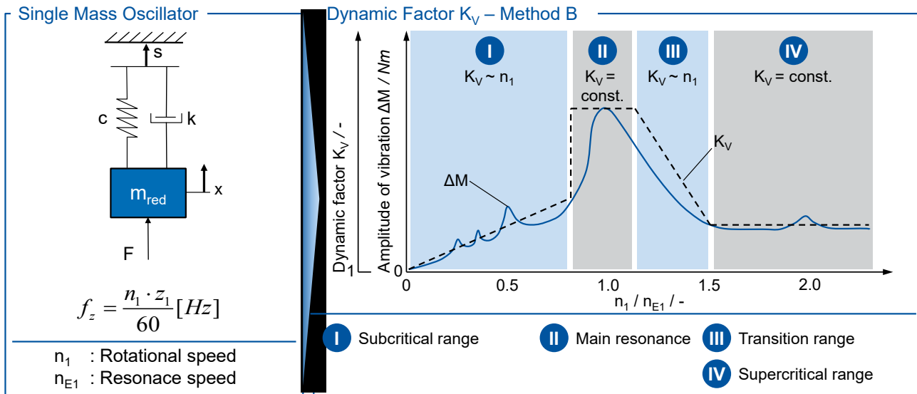
Figure 2-1: Estimation of the additional dynamic loads according to method B of ISO 6336 [ISO19]
