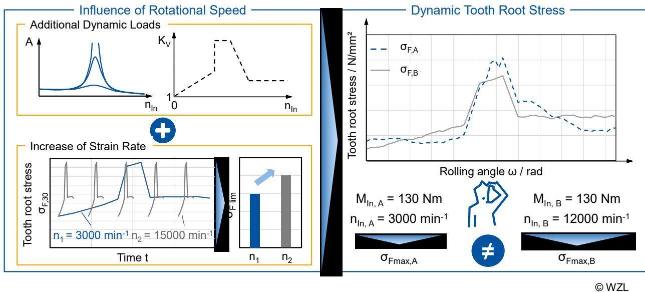
Figure 1-1: Speed influence on the fatigue strength
