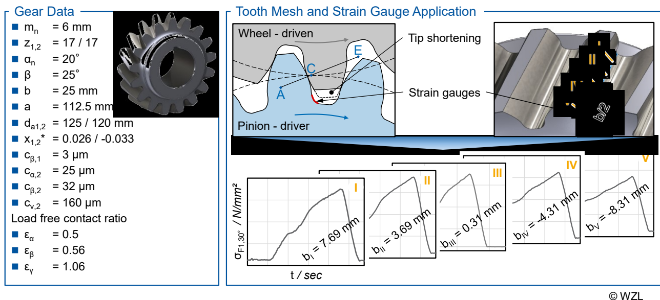
Figure 4-1: Test gear geometry and strain gauge application
