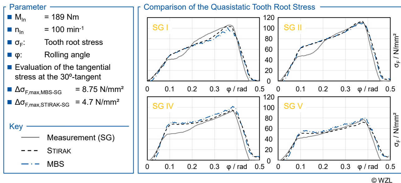
Figure 6-1: Comparison of the calculated and measured tooth root stress in quasi-statics
