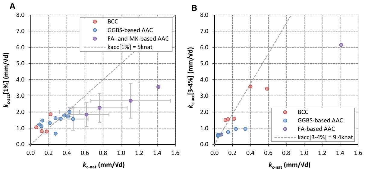
Fig. 7 Carbonation coefficients obtained under accelerated conditions ( A , c_{\text{CO}_2, \text{acc}} = 1\% ; B , c_{\text{CO}_2, \text{acc}} = 3\text{--}4\% ) versus carbonation coefficients obtained under conditions
