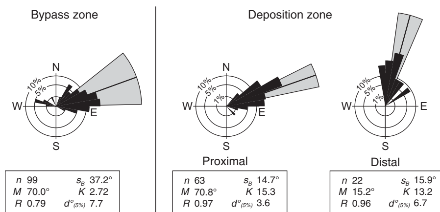
Fig. 13. Equal-area rose diagrams of the palaeoflow measurements in the outcrop complex. Palaeoflow directions in the distal deposition zone deviate from the direction in the proximal deposition zone and in the bypass zone (see Fig. 14 for location). Furthermore, the palaeoflow direction in the bypass zone shows a higher variability than the flows in the lobe. The grey sector describes the mean vector orientation (black line) and length (sector length), and the circular standard deviation (sector width). M : mean vector; R : Mean vector length; S_B : Circular standard deviation; K : Vectorial concentration; d^\circ : Confidence interval of the mean vector. Statistics and equal-area rose diagrams were calculated with EZ-ROSE (Baas, 2000).
