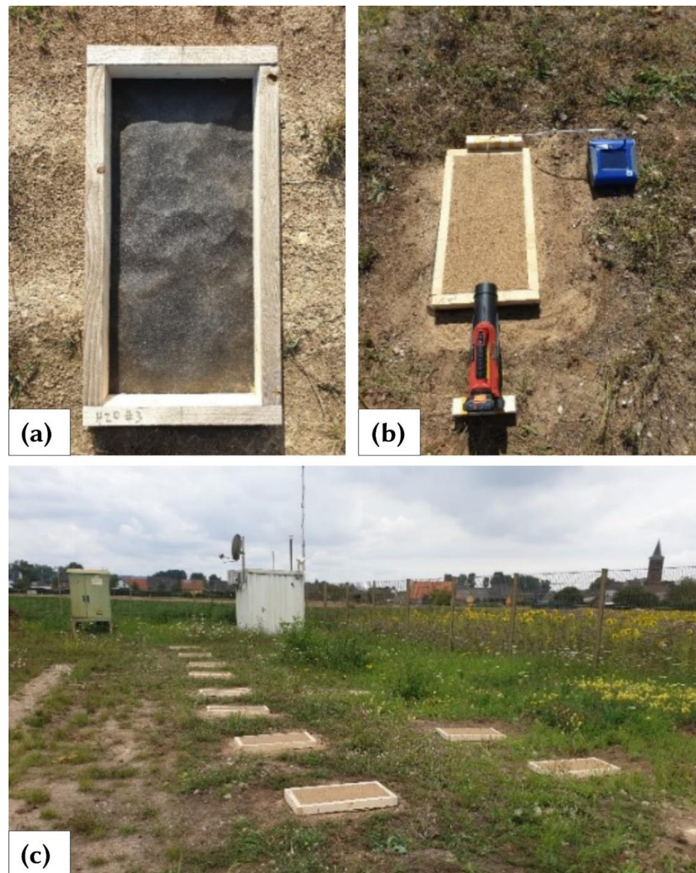
Figure 3. Images of field test site: (a) construction design of individual test plot showing wooden frame and geotextile base, (b) experimental setup of a single test plot with electric blower, isokinetic sampling probe and dust monitor DustTrak DRX 8533 (TSI, Shoreview, USA), and (c) entire test site with installed soil plots and nearby weather station.
