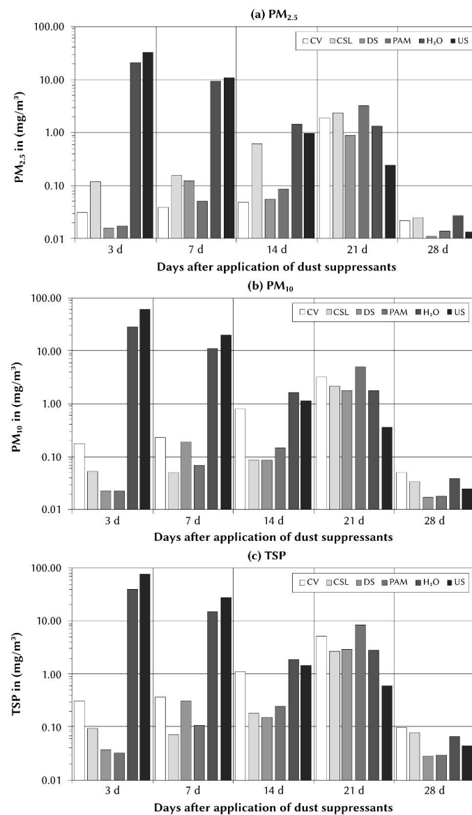
Figure 6. Wind-induced dust emissions from treated and untreated mine soils (mean values, n = 3 ): (a) \text{PM}_{2.5} , (b) \text{PM}_{10} , and (c) TSP. Dust emissions were measured 3, 7, 14, 21, and 28 days after application of dust suppressants. Abbreviations: CV = chicory vinasses, CSL = corn steep liquor, DS = decantation syrup, PAM = palatinose molasses, \text{H}_2\text{O} = water-treated soil, US = untreated soil.
