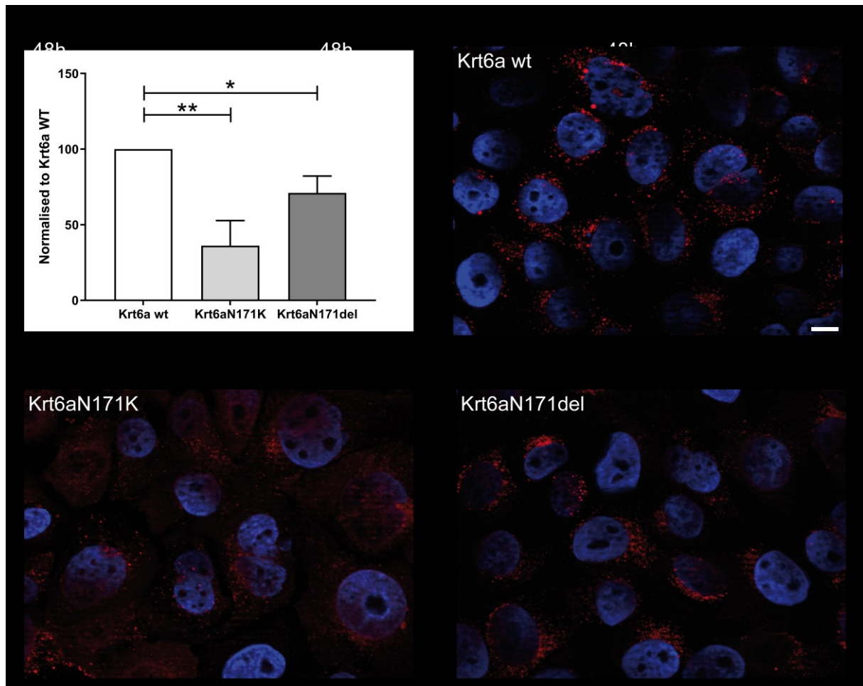
Figure 43- Lysosomal function is reduced in Pachyonychia congenita keratinocytes. To assess lysosomal function in terms of cathepsin B function, the cells were incubated for 60 minutes with Magic Red® Cathepsin B substrate. Differentiated wt (b), Krt6aN171K (c) and Krt6aN171del (d) cells display a red fluorescence signal in lysosomes (contrast was equally set for images taken on the same day, i.e. both PC mutants). Three independent experiments with n=327 (wt), n=216 (Krt6aN171K), and n=241 (Krt6aN171del) were performed. The red fluorescence signal was measured as area percentage per cell, and the values were normalised to wt cells for each replicate. Note the significantly reduced fluorescent signal in both PC cell lines (a). Scale bar = 10 \mu m. Comparisons between groups were performed using one-way ANOVA with Holm Šidák post-test. * p < 0.05 , ** p < 0.01 .
