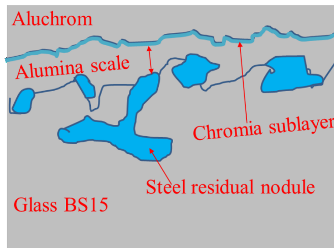
Fig. 4-67. Schematic diagram of the interface reaction between BS15 glass sealant and Aluchrom joined at 1075 °C for 5 min
