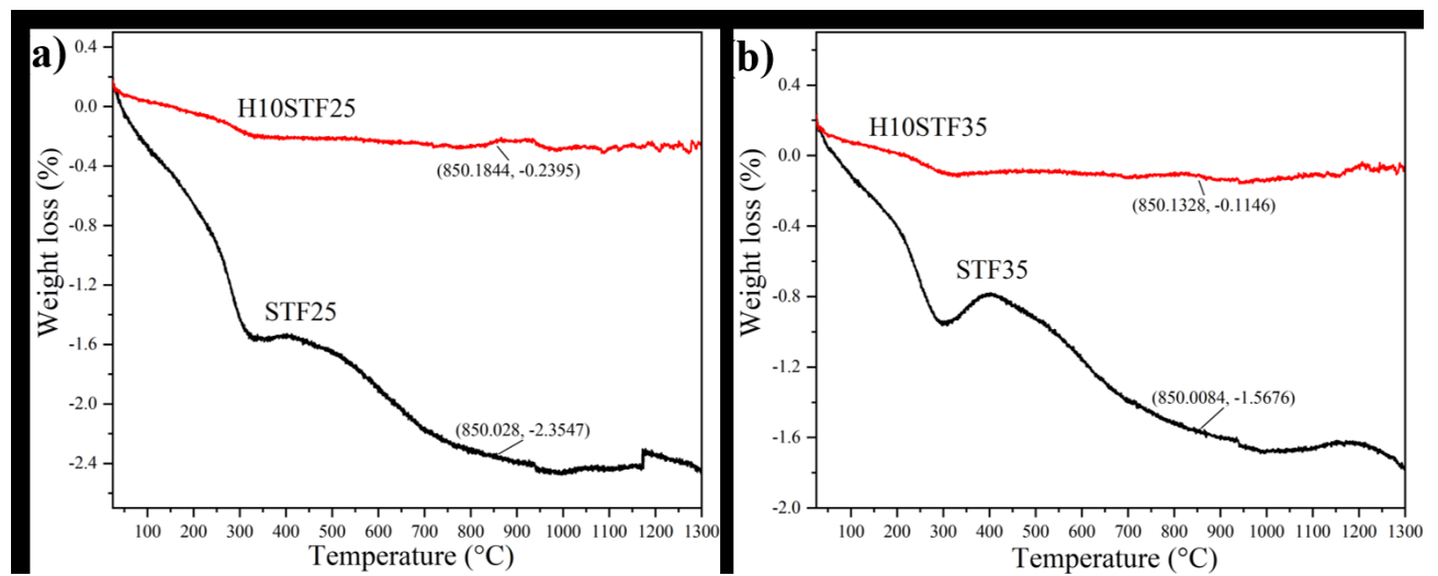
Fig. 4-10. Weight loss curves of STF fillers and mixed with glass H
