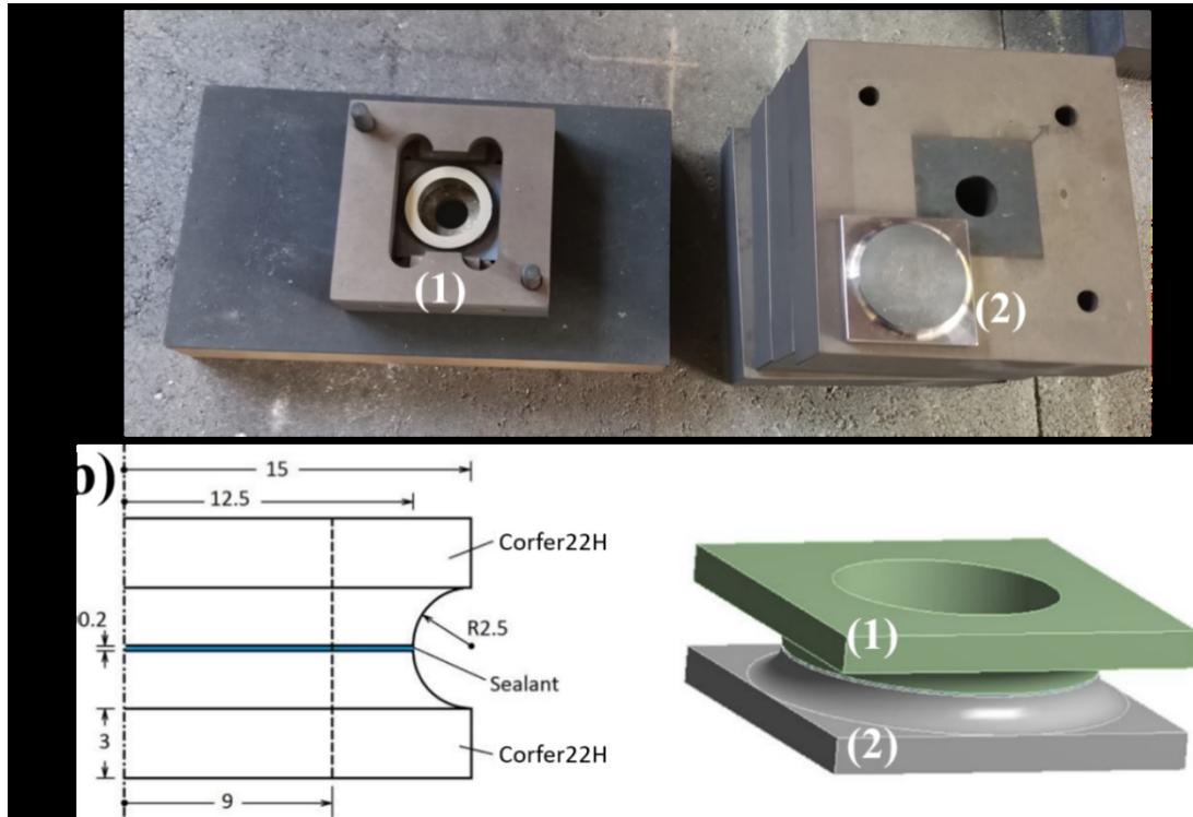
Fig. 3-6. (a) Assembling of hourglass shaped torsion specimen process, sealant was placed in the middle of two Crofer22H plates for further joining at 850 °C for 10 h under a deadload 3900 \pm 100 g; (b) schematic of the hourglass shaped specimens [125] after joining, the dimensions are in mm. (1) is Crofer22H plate with an inner hole of \varnothing 18 mm and green foil of sealant applied to it (2) is opposite Crofer22H plate without hole.
