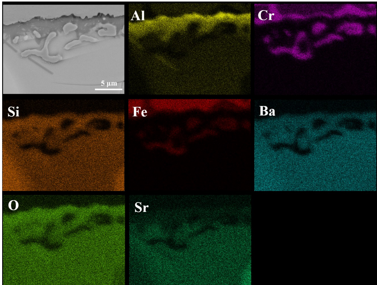
Fig. 4-66. SEM-EDS maps of the gas-tight joint Alchrom/BS15/Aluchrom joined at 1075 °C for 5 min to analyze interaction between BS15 glass and Aluchrom
