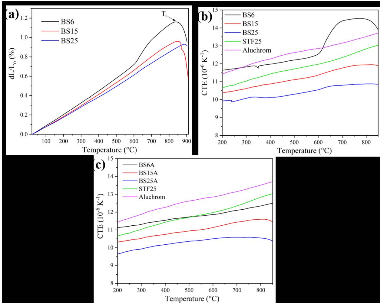
Fig. 4-56. Dilatometer curves of BS glasses, (a) elongation plots, dilatometer softening temperature ( T_s ), (b) CTE of BS glasses as a function of temperature comparing with membrane STF25 and Aluchrom, (c) dilatometer curves of the annealed BS samples after 850 °C for 50 h
