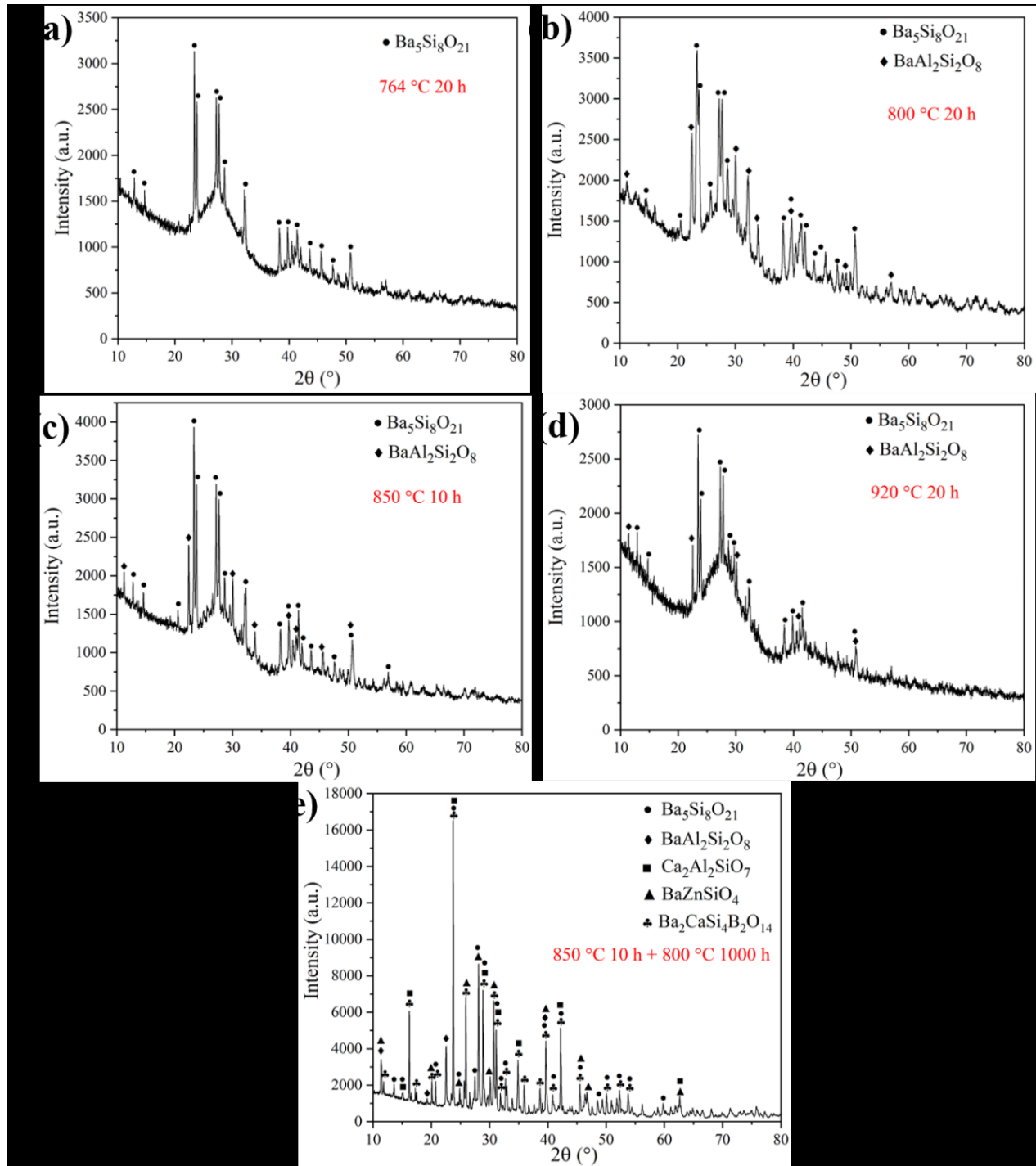
Fig. 4-4. Glass H after different heat-treatments for crystallization analysis, (a) XRD pattern of glass H after heating at 764\text{ }^\circ\text{C} for 20 hours, (b) XRD pattern of glass H after heating at 800\text{ }^\circ\text{C} for 20 hours, (c) XRD pattern of glass H after heating at 850\text{ }^\circ\text{C} for 10 hours, (d) XRD pattern of glass H after heating at 920\text{ }^\circ\text{C} for 20 hours, (e) XRD pattern of glass H after heat-treatment at 850\text{ }^\circ\text{C} for 10 hours followed by 800\text{ }^\circ\text{C} for 1000 hours, with same heating and cooling rate of 2\text{ }^\circ\text{C}/\text{min} .
