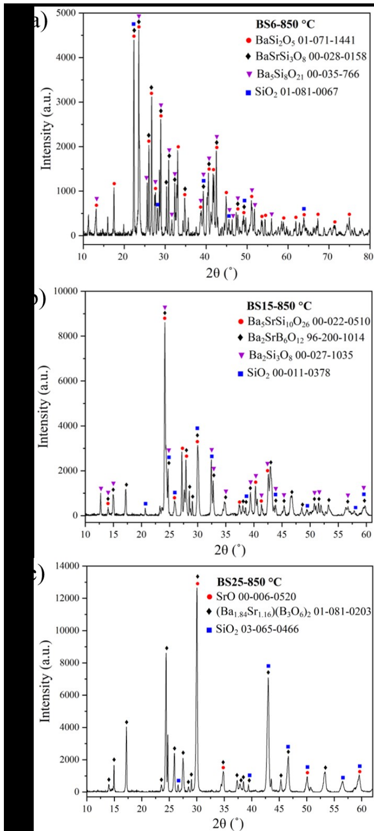
Fig. 4-59. XRD patterns of BS glasses heated at 850 °C for 50 h, (a) BS6, (b) BS15 and (c) BS25
