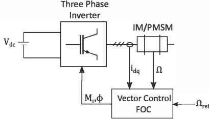
Fig. 1: Electrical system layout
