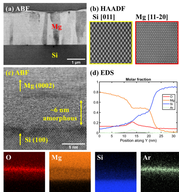
Fig. 3 Cross-sectional (a) ABE-STEM micrograph of columnar Mg grains, (b) atomically-resolved HAADF-STEM micrograph of the Si substrate and the selected Mg grain along [2110], and (c) high resolution ABE-STEM micrograph of the interface between Mg and Si; (d) EDS elemental maps of the area imaged in (c) and the integrated line profile of the molar composition.
