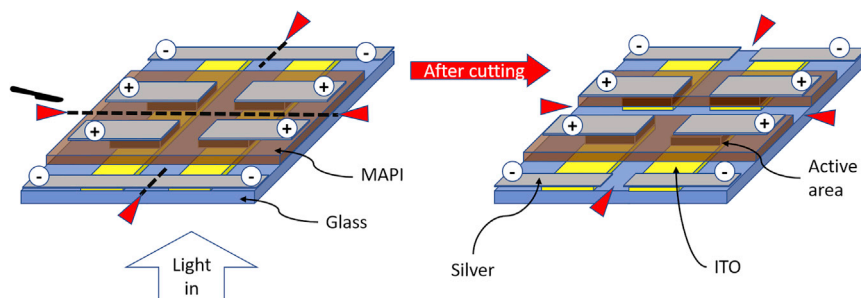
Figure 3. Solar module cut scheme
