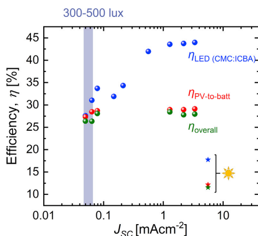
Figure 8. Module efficiency ( \eta_{LED} ), charging efficiency ( \eta_{PV-to-batt} ), and overall efficiency ( \eta_{overall} ) versus short-circuit current density of the solar module under LED illumination 300–500 lux LED intensity has been highlighted in blue gray. AM1.5G results have been plotted as stars for comparison.
