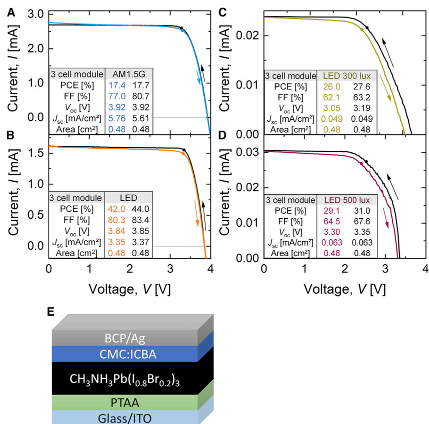
Figure 2. Illuminated current voltage curves for the CH 3 NH 3 Pb(I 0.8 Br 0.2 ) 3 module
