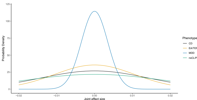
Figure 2. Estimated effect-size distributions for risk SNPs associated to esophageal atresia with or without tracheoesophageal fistula (EA/TEF), non-syndromic cleft lip with or without cleft palate (nsCL/P), major depressive disorder (MDD), and Crohn's disease (CD) according to GENESIS (Zhang et al. 43 ). The GWAS data for MDD and CD were drawn from GENESIS and represent extreme phenotypes for diseases with high and low polygenicity. In addition to EA/TEF, GWAS data on nsCL/P was used as another developmental disorder. The x axis represents the joint effect sizes of disease-contributing SNPs, while the y axis shows their probability density of joint effect sizes. Distributions with flatter tails imply that the underlying diseases have relatively greater numbers of risk SNPs with larger effect size.
