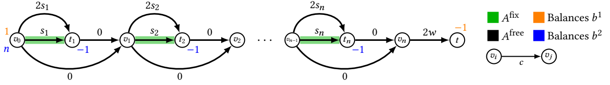
Figure 2: Construction of RobT≡ instance \tilde{I} .
