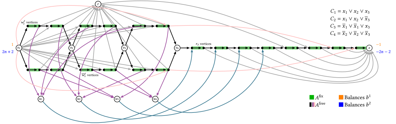
Figure 1: Construction of RobT≡ instance \tilde{I} .
