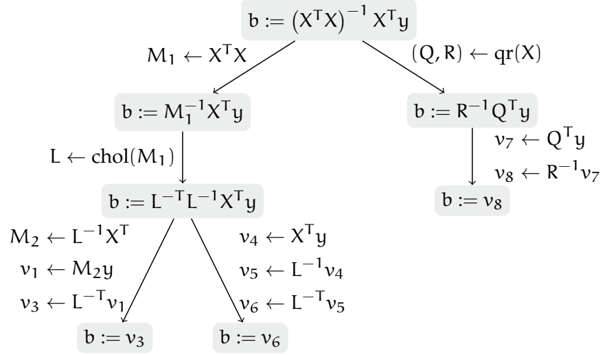
Figure 4.1: An example of a search graph for the input b := (X^T X)^{-1} X^T y . This graph represents only a small part of the search space that Linnea actually explores.
