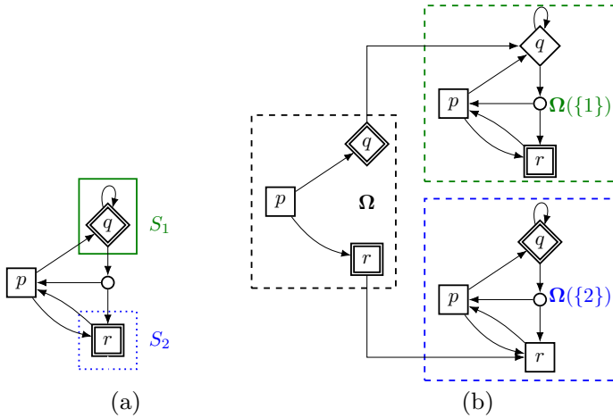
Fig. 2 a SG with non-absorbing lex-objective \Omega = (\text{Reach}(S_1), \text{Reach}(S_2)) . b The three stages identified by the sub-objectives \Omega , \Omega(\{1\}) = \text{Reach}(S_2) , and \Omega(\{2\}) = \text{Reach}(S_1) . The latter two stages are simple
