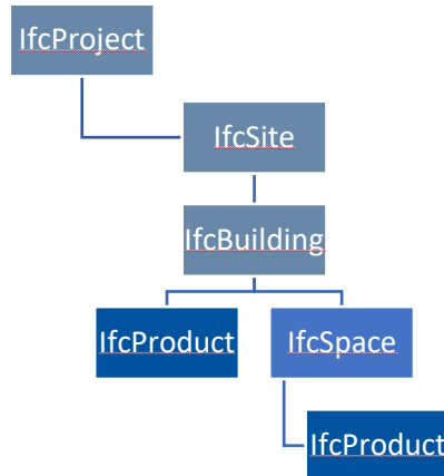
Fig. 14: IFC Spatial Tree showing model hierarchy.
