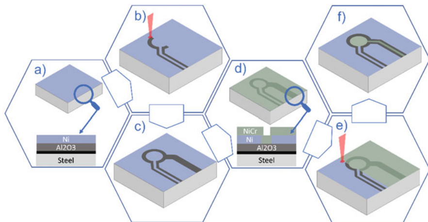
Fig. 7 The interplay between laser ablation and PVD coating. (a) The steel substrate is PVD coated with an interlayer, Al 2 O 3 , and Ni. (b) Selective laser ablation of Ni to form an isolated path. (c) Resulting ablation pattern. (d) PVD coating with NiCr. (e) Laser ablation of NiCr. (f) The finished thin film sensor with a Ni and a NiCr conductor, which meet at one point to form a sensor
