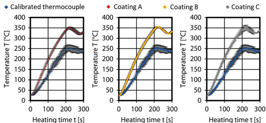
Fig. 4 Temperature measurement by PVD sensor coatings A, B, and C
