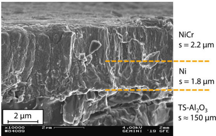
Fig. 6 PVD Ni + NiCr sensor on TS insulation coating in SEM cross-fraction
