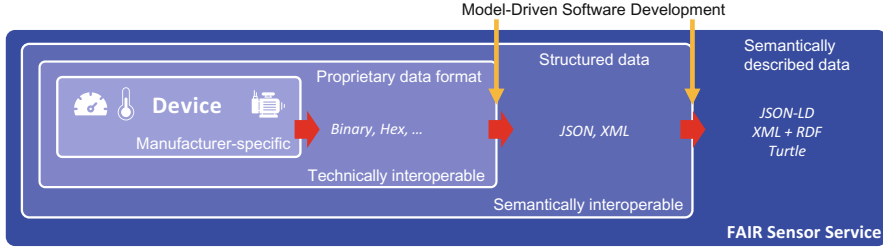
Fig. 3 Our proposed interoperability hierarchy of interfaces for Cyber-Physical Measuring System (CPMSs). While manufacturer-specific interfaces are mostly non-interoperable, we can achieve interoperability by providing context information through semantically annotated (meta)data
