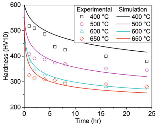
Fig. 8 Comparison of experimental and simulated hardness for tempered medium manganese steel
