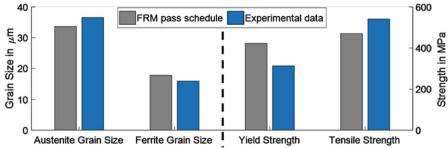
Fig. 7 Comparison between the measurements and FRM-predicted values
