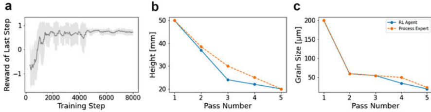
Fig. 11 (a) Training progress of a SAC agent on the rolling task shown as the rolling mean of the received reward with the shaded region showing the rolling standard deviation. (b) Height and (c) grain size of material throughout pass schedule generated by a trained RL agent and a pass schedule created by a process expert. (Adapted from Scheiderer et al. 2020)
