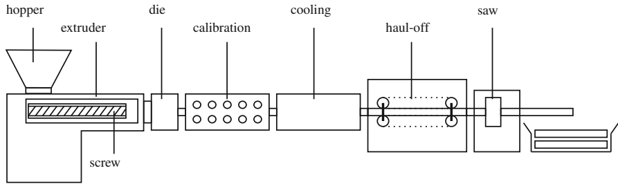
Fig. 2 Process sections in a classic extrusion process (Hilger and Hosters 2022)
