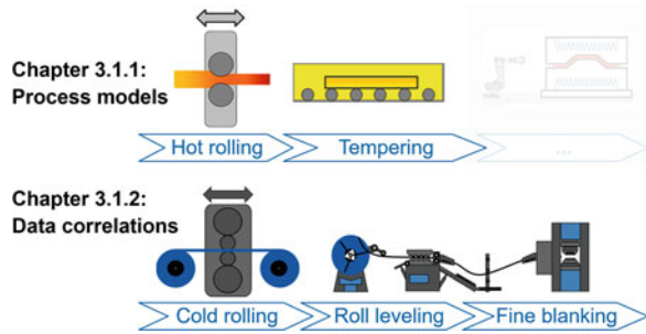
Fig. 6 Selected processes of the metal processing process chain
