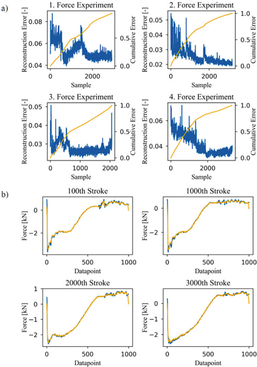
Fig. 10 (a) The (cumulated) reconstruction errors are presented. (b) Selected strokes of the second experiment are presented that are representative for the change in the force signal of the stripping segments (Niemietz et al. 2021)
