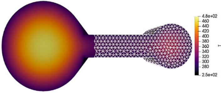
Fig. 4 Exemplary computational mesh and corresponding FEM solution of the temperature distribution in an extruded profile
