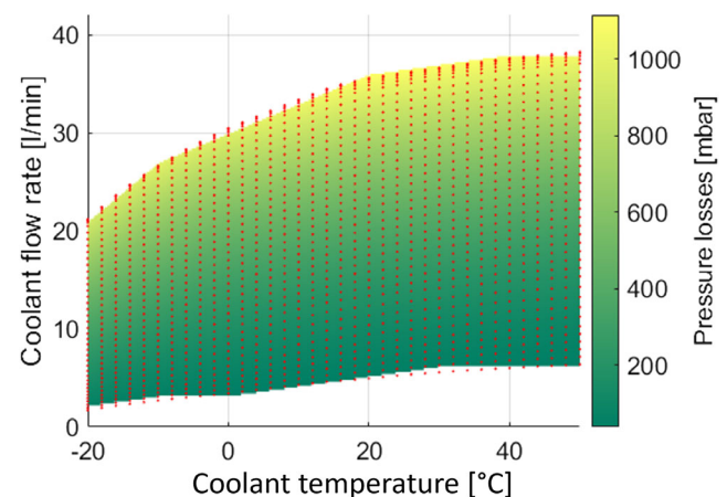
Figure 8. Data-based pressure losses outside of the cooling plate depending on volume flow rate and coolant temperature.
