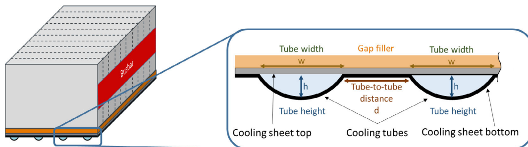
Figure 5. Schematic representation of the cooling plate with multiple geometric design parameters.
