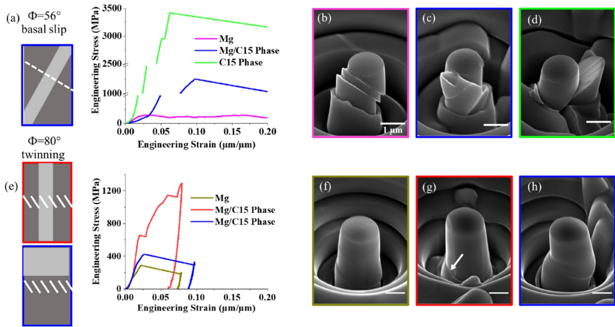
Figure 6: (a) Engineering stress strain curves of micropillars oriented for basal slip containing \alpha -Mg phase, \alpha -Mg/CaAl 2 phase mixture, and CaAl 2 phase. (b), (c), and (d) are the micrographs of micropillars containing \alpha -Mg phase, \alpha -Mg/CaAl 2 , and CaAl 2 phase, respectively. Both (b) and (c) were milled into the same Mg grain which has high Schmid factor for basal slip. (e) Engineering stress strain curves of micropillars containing the \alpha -Mg phase ( \phi=80^\circ ) and a Mg/CaAl 2 interface (f), (g) and (h) are the SE images of the deformed micropillars. The frame colours of (f), (g) and (h) correspond to the respective stress-strain curves. The white arrow in (g) highlights the point of slip transfer from Mg to CaAl 2 . Scale bars represent the length of 1 \mu\text{m} .
