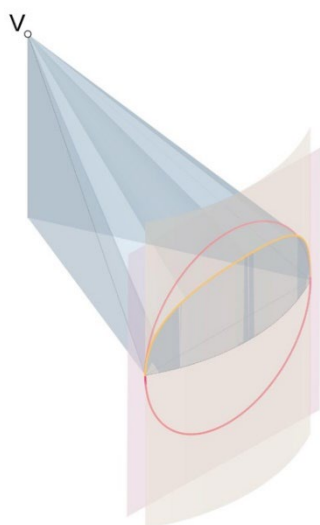
Figure 12. Circular conoidic surface with director plane.
