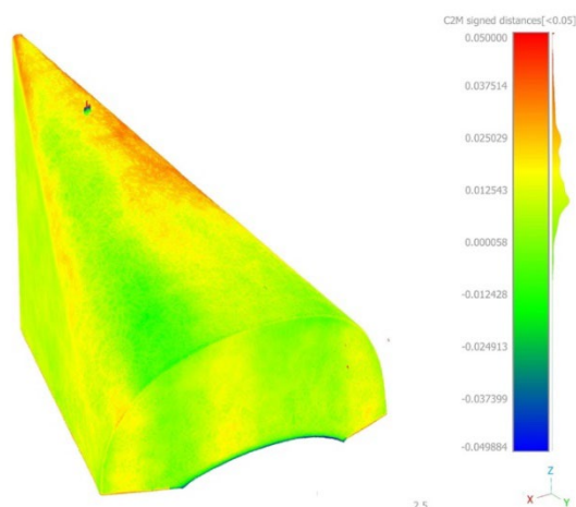
Figure 15. Cloud-to-mesh distance (in the range of -5cm to 5cm) between the captured point cloud and the reconstructed geometry of the cone.
