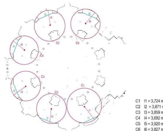
Figure 11. Conic vaults, pillars and construction of the circle chord
