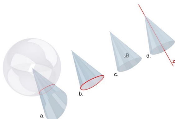
Figure 16. Construction of the axis of a quadric cone: a) Intersection between the cone and a generic sphere. b) The intersection curve (in red). c) The barycentre of the resulting cone (B). d) Construction of the axis of the cone (z).
