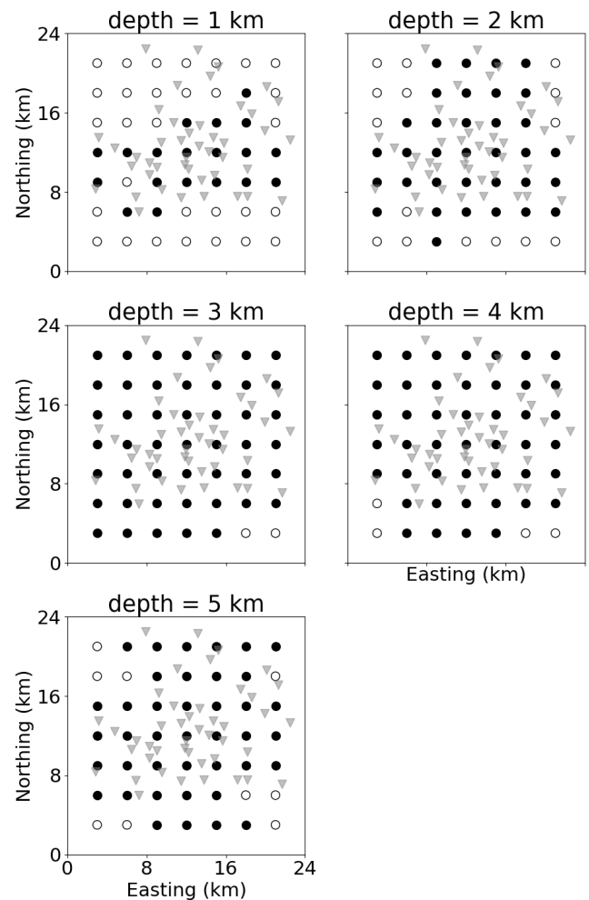
Figure 7. Successful locations with TRI (filled circles) appear in the centre of the model and beneath the seismic stations (grey triangles). Unsuccessful locations (open circles) appear mainly at the borders and at shallow and deep depths.
