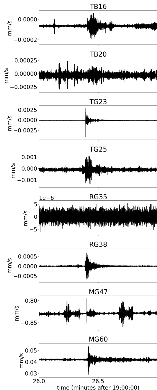
Figure 5. Traces on network stations recording on 5 May 2022. Traces are filtered between 10 and 50 Hz around the time of detected and located event in Eschweiler (308 894 m easting, 5 629 087 m northing, close to station RG38) on 5 May 2022, 19:26:21.7 UTC with a magnitude of M_L 1.1 (Earthquake Observatory Bensberg University Cologne, 2022).
