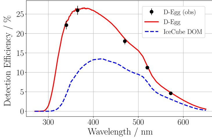
Figure 4. Detection efficiency at the threshold of 0.25 PE (photoelectrons) as a function of wavelength. The black markers show the values of the glass and silicone transparency measured in the laboratory convoluted with the averaged PMT QE provided by HPK. The red line represents a convolution of the average PMT quantum efficiencies from HPK with the glass and silicone transmittance measured by Okamoto Glass and Shin-Etsu Silicone, respectively, for the D-Egg. The blue line indicates the same quantity for the IceCube DOM as a reference.
