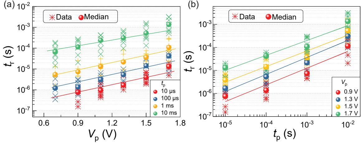
Figure 6.2: (a) The statistical analysis of t_r as a function of (a) V_p and (b) t_p collected from 10 measurements for each V_p/t_p combination. Reproduced with permission from [1].
