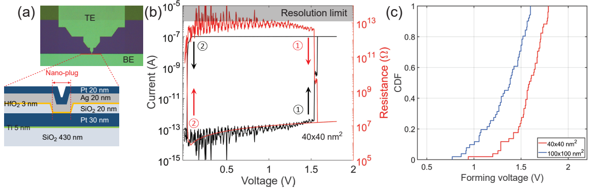
Figure 4.11: (a) Top panel: optical microscopy image of the nano-structured plug-type device. Bottom panel: a schematic cross-sectional view of the red-colored line in the top panel. (b) Typical forming curve of the HO3P|Pt plug-type device with cell dimension of 40 nm x 40 nm. The current response is plotted in black while the calculated resistance of the cell is plotted in red. (c) CDF plot of the forming voltage collected from 50 cells each for 40 nm x 40 nm and 100 nm x 100 nm devices. A current compliance of 100 nA was used during the measurement to prevent current overshoot.
