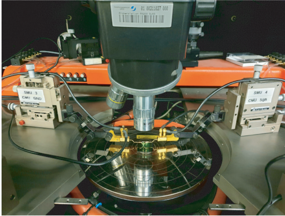
Figure 3.12: Photo of the Sues MicroTec PA-200 semi-automatic table.
