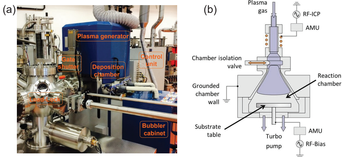
Figure 3.3: Left: Photo of the FlexAL TM ALD system. Right: Cross-section of the ALD chamber, modified from [158].
