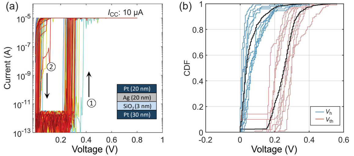
Figure 4.23: I - V sweep of the SO3P|Pt device measured under a compliance current ( I_{CC} ) of 10 \mu A. (b) Statistical distribution of the hold ( V_h ) and threshold ( V_{th} ) voltages collected from 10 devices and 100 cycles each.
