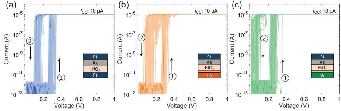
Figure 4.19: Typical threshold I - V curves for (a) HO3P|Pt, (b) HO3P|TiN, and (c) HO3P|W devices. The \text{TiO}_x and \text{WO}_x interfacial oxides are shown with light orange and light green colors, respectively. A sweep rate of 62.5 mV/s was used for the measurements. Reproduced with permission from [3].
