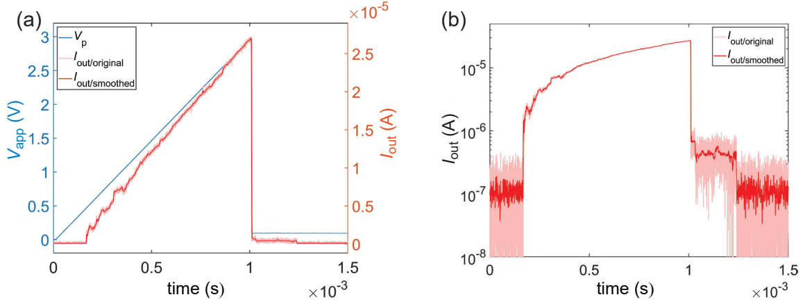
Figure 6.10: (a) The triangular pulses scheme used to analyze the influence of sweep rate on the relaxation time. The voltage pulse V_p is given in blue and the output current I_{out} in red. (b) A \log(I_{out}) - t plot of the data in (a) showing the original and smoothed data using Gaussian-weighted filter.
