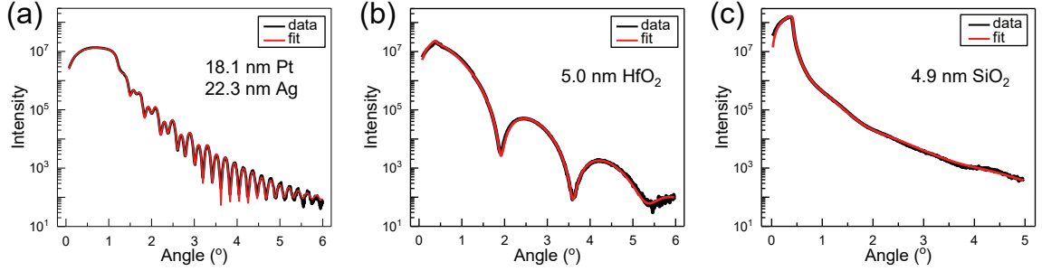
Figure 3.8: X-ray reflectivity measurements of different layers. (a) Sputter deposited Ag metal film on \text{SiO}_2 substrate. (b) ALD grown \text{HfO}_2 film on \text{SiO}_2 substrate. (c) ALD grown \text{SiO}_2 film on Si substrate.
