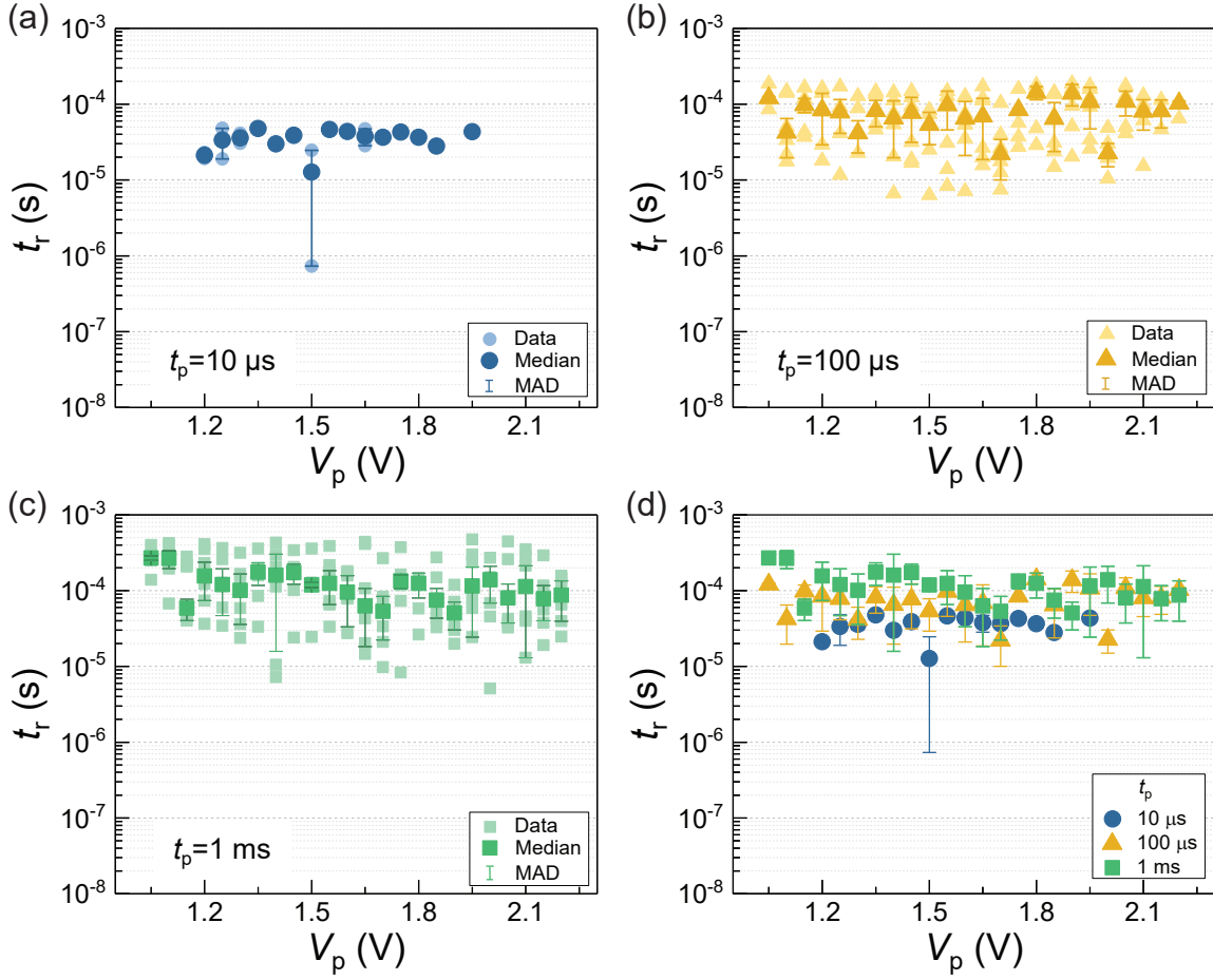
Figure 6.13: Relaxation time plotted as a function of V_p for various t_p of (a) 10 \mu s , (b) 100 \mu s , and (c) 1 ms . (d) Median of t_r as a function of V_p . The median values and median absolute deviations (MAD) of the experimental data are displayed using color-filled symbols and vertical lines, respectively. A 100 k\Omega resistor was used during the measurements.
