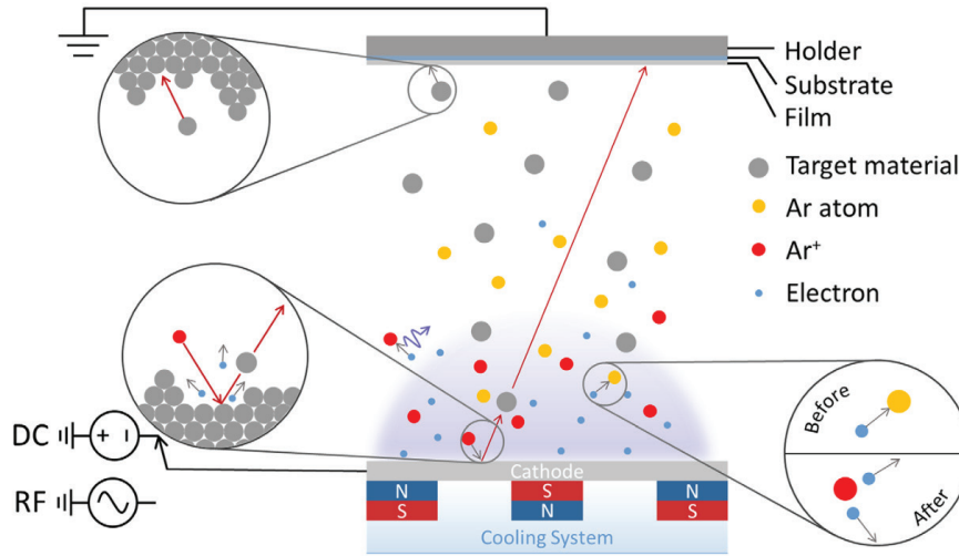
Figure 3.6: Basics of sputter process. Adapted from [160].
