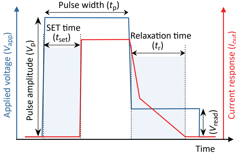
Figure 5.1: Various terminologies and the definitions of SET time ( t_{\text{set}} ) and relaxation time ( t_r ) from a temporal response measurement in the time domain. The applied voltage ( V_{\text{app}} ) and output current signal ( I_{\text{out}} ) are shown in blue and red colors, respectively. Reproduced with permission from [1].
