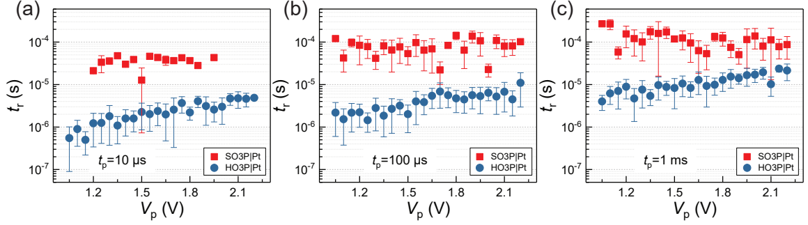
Figure 6.14: Relaxation dynamics of HO3P|Pt and SO3P|Pt devices. The median of t_r is plotted against V_p for various pulse durations of (a) 10 \mu s, (b) 100 \mu s, and (c) 1 ms.
