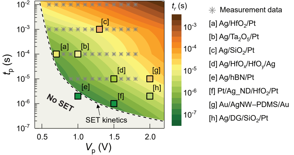
Figure 7.2: A heat map of the combination of the SET kinetics (broken line) and relaxation dynamics showing several orders of magnitude change in relaxation time t_r over a certain range of V_p and t_p . The SET kinetics curve is a representative fitting curve of the experimental data. The color-coded relaxation time is plotted based on experimental data (represented by stars) and an extrapolation from the fitting of the experimentally obtained data. Letter assigned boxes are t_r data collected from various publications of [35, 60, 174, 190, 204–207]. Reproduced with permission from [1].
