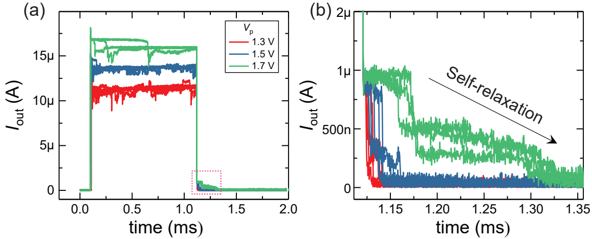
Figure 6.1: (a) Typical current response, I_{out} - t , under programming pulses V_p/ t_p of 1.3 V, 1.5 V, and 1.7 V/ 1 ms followed by a 0.1 V monitoring voltage. (b) Magnified plot of the pink marked region in (a), showing the different relaxation times for different V_p . R_{series} of 100 k \Omega was used during the measurement. Reproduced with permission from [1].
