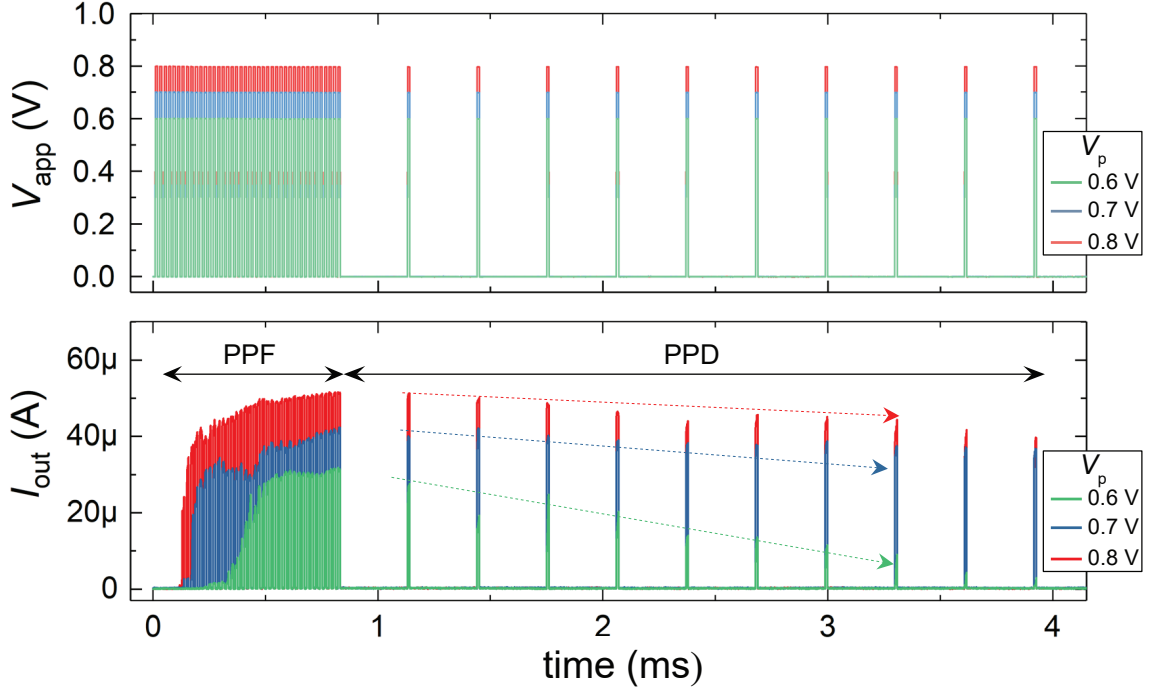
Figure 8.3: PPF and PPD of a HO3P|Pt diffusive memristor under a continuous pulse train with varying V_p of 0.6 V, 0.7 V, and 0.8 V, and two pulse intervals t_{int} of 10 \mu s and 500 \mu s, with a fixed t_p of 10 \mu s.
