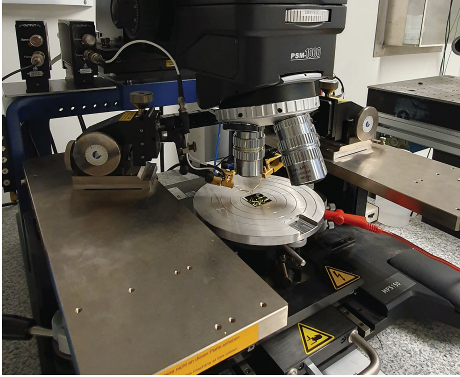
Figure 3.13: Photo of the Keithley 4200-SCS measurement setup.
