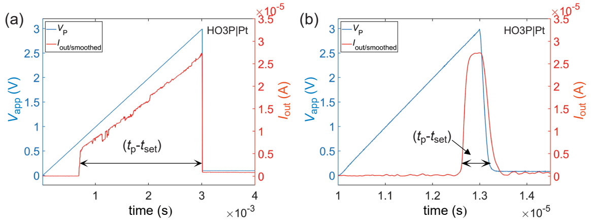
Figure 6.12: (a) An output current I_{out} from a triangular pulse scheme plotted for HO3P|Pt device measured under t_p of (a) 3 ms (b) 3 \mu s. The excessive pulse is shown as t_p - t_{set} .
