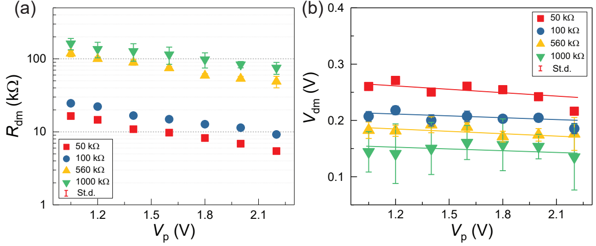
Figure 6.9: Calculated (a) cell resistance R_{dm} and (b) voltage drop across the cell V_{dm} plotted as against V_p for different R_{series} values at a fixed t_p of 1 ms. The lines in (b) are a guide to the eye. Reproduced with permission from [2].
