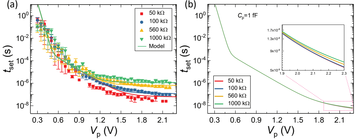
Figure 5.9: (a) Simulation of the SET kinetics when an RC -time constant of the circuit is considered with C_p = 1.15 pF. (b) Simulation data was obtained with C_p of 1 fF, showing faster switching times and negligible differences between the R_{\text{series}} values. Inset shows a magnified image of the pink box in (b). Reproduced with permission from [2].
