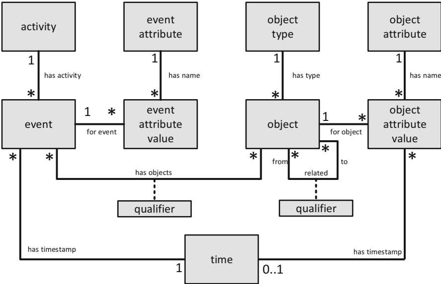
Fig. 3 Process mining metamodel: events have a timestamp, an activity, and other event attributes. An event may refer to any number of objects. Each object has a type and attributes that may change over time
