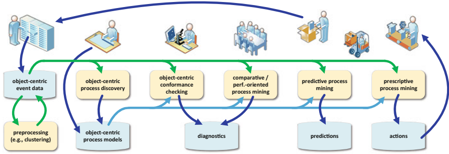
Fig. 4 The process mining pipeline showing the different types of artifacts and data processing steps starting from object-centric event data
