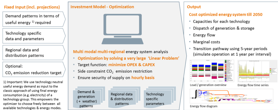
Fig. 2 Overview of the multi-modal investment and operation model (MIM)
