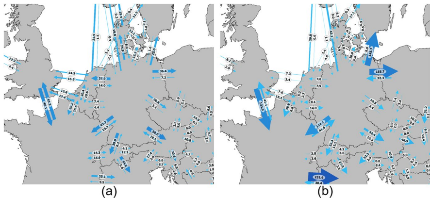
Fig. 13 Annual aggregated exchange flows (in TWh): a Results of the base scenario. b Results of the copper plate scenario
