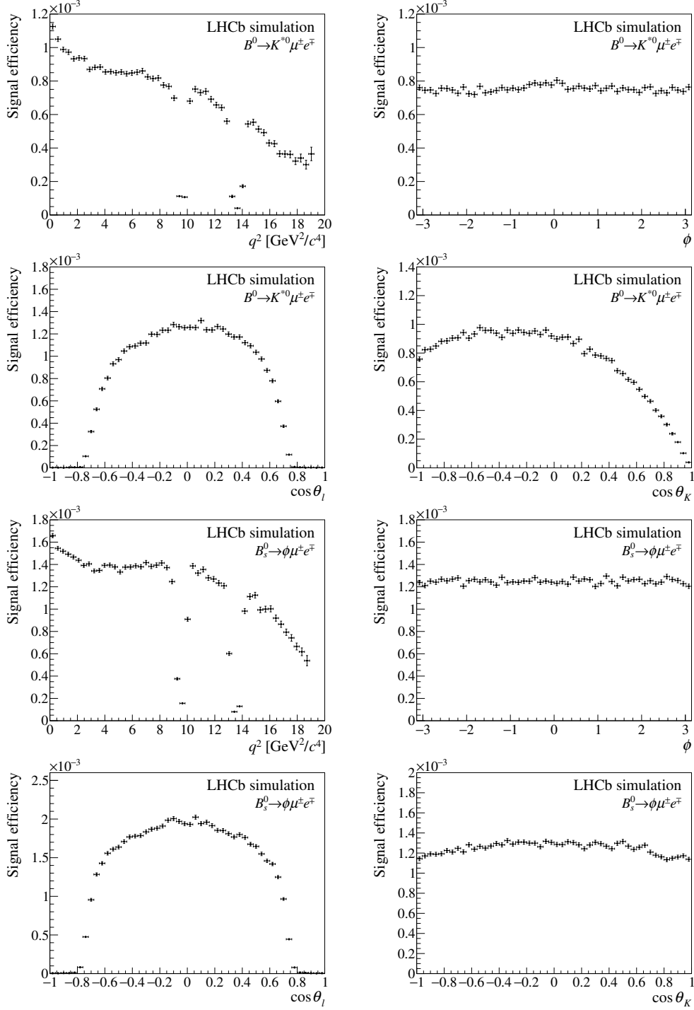
Figure 5. Reconstruction and selection efficiency, combined for the 2011–2018 samples, for (top) B^0 \rightarrow K^{*0} \mu^\pm e^\mp and (bottom) B_s^0 \rightarrow \phi \mu^\pm e^\mp signal decays depending on q^2 and the three decay angles \cos \theta_\ell , \cos \theta_K , and \phi . The selection efficiency drops in the q^2 region around the J/\psi and \psi(2S) masses as a result of the veto against misidentified backgrounds.
