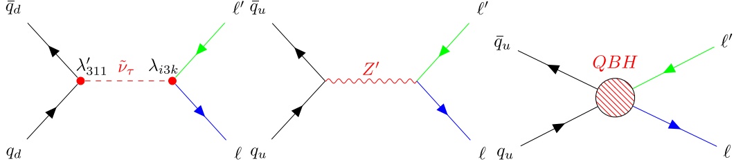
Figure 1. Leading order Feynman diagrams considered in our search. Left: Resonant production of a \tau sneutrino in an RPV SUSY model that includes the subsequent decay into two leptons of different flavors. The \tilde{\nu}_\tau is produced from the annihilation of two down quarks via the \lambda'_{311} coupling, and then decays via the \lambda couplings. Middle: Resonant production of a Z' boson with subsequent decay into two leptons of different flavors. Right: Production of quantum black holes in a model with extra dimensions that involves subsequent decay into two leptons of different flavors.
