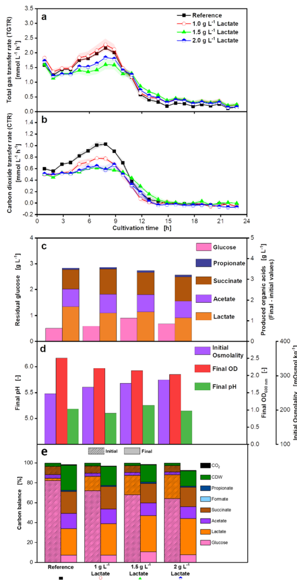
Fig. 6 Effect of initial lactate addition to P. vulgatus shake flask cultivations in duplicates. Medium = DMMG, c_{\text{Glucose}} = 6 \text{ g L}^{-1} , c_{\text{buffer}} = 50 \text{ mM MOPS} , T = 37^\circ \text{C} , n = 100 \text{ rpm} , V_L = 50 \text{ mL} , initial \text{OD} = 0.35 , initial pH after inoculation = 7.23, \text{vvm} = 0.2 \text{ min}^{-1} , gas mix = 1% \text{CO}_2 and 99% \text{N}_2 . Online data of a total gas transfer rate (TGR) and b carbon dioxide transfer rate (CTR) shadows indicate maximum and minimum values of duplicates (error bars). Offline data of c produced organic acids including propionate, succinate, acetate and lactate, and remaining glucose; d initial osmolality, final \text{OD}_{600\text{nm}} and final pH as mean values of biological duplicates. Samples to measure initial osmolality were drawn immediately after inoculation. Samples to measure final \text{OD}_{600\text{nm}} , final pH, and HPLC analysis were drawn immediately after termination of the experiment, indicated by the last online data point in a and b . e Molar carbon balance in % of the initial carbon, calculated with Eqs. 3-5. Initial values include acids from preculture. The corresponding molar carbon balance in \text{mmol}_C \text{ L}^{-1} can be found in Supplementary Fig. S4
