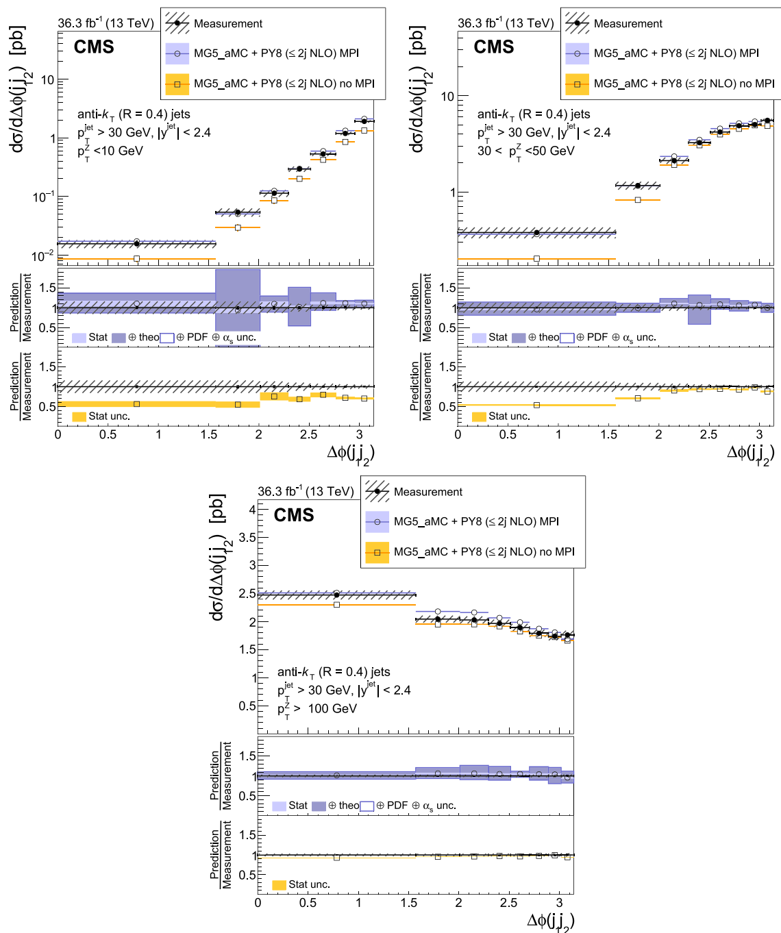
Fig. 8 Cross section as a function of \Delta\phi(j_1j_2) between two leading jets in three p_{T(Z)} regions: p_{T(Z)} < 10 GeV (upper left), 30 < p_{T(Z)} < 50 GeV (upper right), p_{T(Z)} > 100 GeV (lower). The error bars on the data points represent the statistical uncertainty of the mea-
