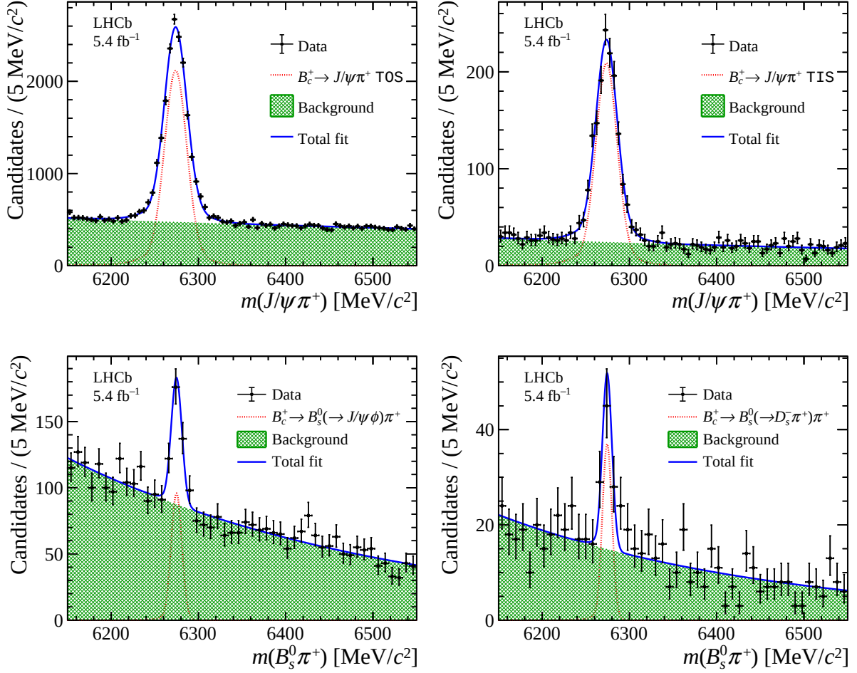
Figure 1: Invariant-mass distributions of B_c^+ candidates: (top left) B_c^+ \rightarrow J/\psi \pi^+ TOS, (top right) B_c^+ \rightarrow J/\psi \pi^+ TIS, (bottom left) B_c^+ \rightarrow B_s^0(\rightarrow J/\psi \phi) \pi^+ , and (bottom right) B_c^+ \rightarrow B_s^0(\rightarrow D_s^- \pi^+) \pi^+ . The black dots represent the data, the blue line represents the results of the total fit, and the red dashed line and green shaded area show the signal and combinatorial background components, respectively.
