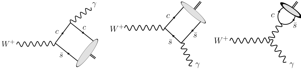
Figure 1: Tree-level Feynman diagrams for the decay W^+ \rightarrow D_s^+\gamma .
