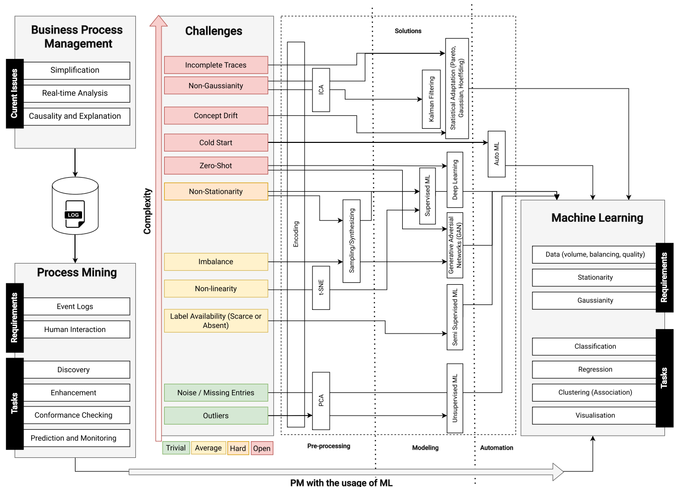
FIGURE 4. From task to task, an overview of PM and ML relationship.
