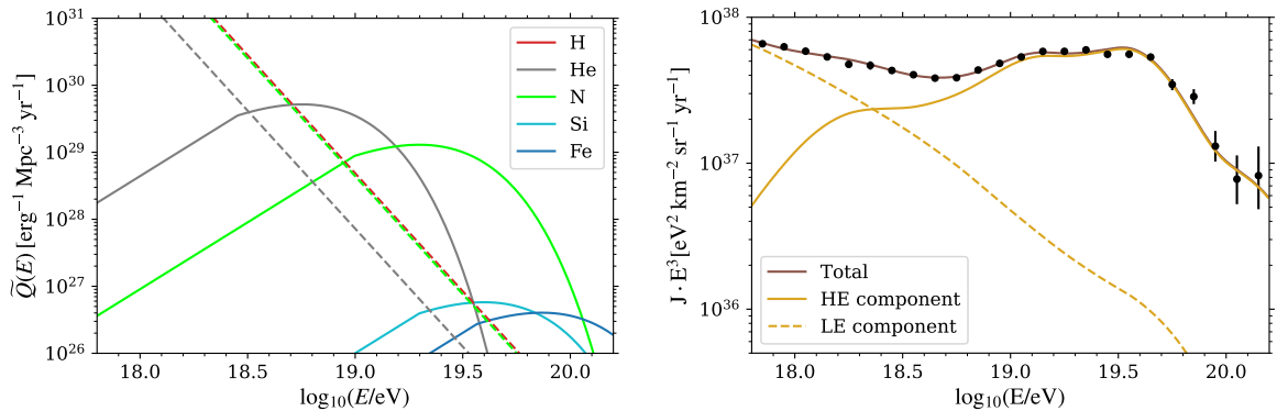
Figure 4. SCENARIO 2. Left: the generation rate at the sources for each representative mass; the LE and HE contributions are shown as dashed and solid lines, respectively. Right: the corresponding best fit results for the all-particle energy spectrum at the Earth, given by the superposition of the LE and HE extragalactic components.
