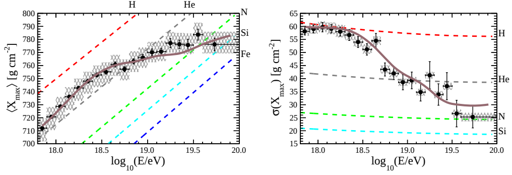
Figure 3. SCENARIO 1. First two moments of the X_{\max} distributions as predicted by the best-fit results, along with the measured values and the predictions for pure compositions of various nuclear species according to EPOS-LHC (dashed lines).
