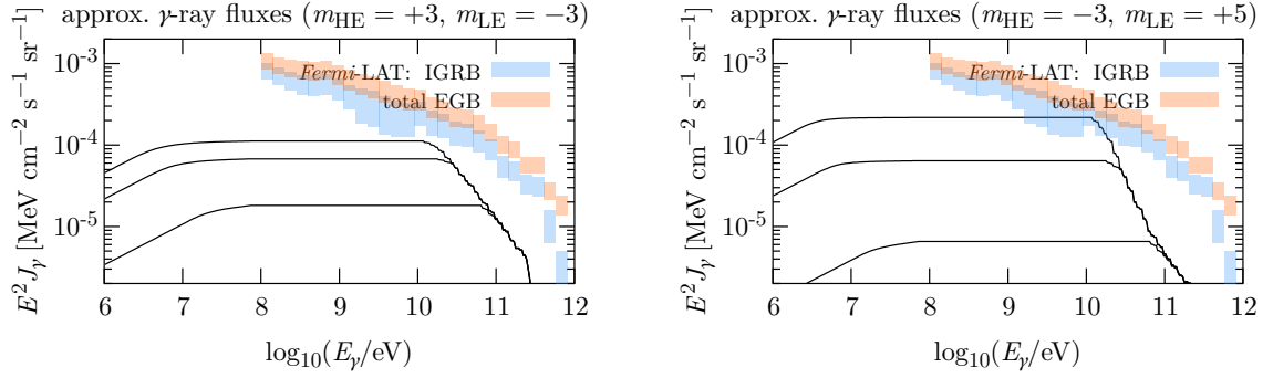
Figure 16. Fluxes at Earth of gamma-ray cascades produced in UHECR propagation in two example scenarios with (from bottom to top) z_{\max} = 1, 3 and 5 , estimated through the analytic approximation from Ref. [110], and compared to Fermi -LAT measurements from Ref. [111] (with error bands showing uncertainties due to those on Galactic foreground models). Note that this approximation is not very accurate for short source distances, and hence for high photon energies. All other scenarios in Section 5 with D \lesssim 1000 result in similar or lower fluxes.
