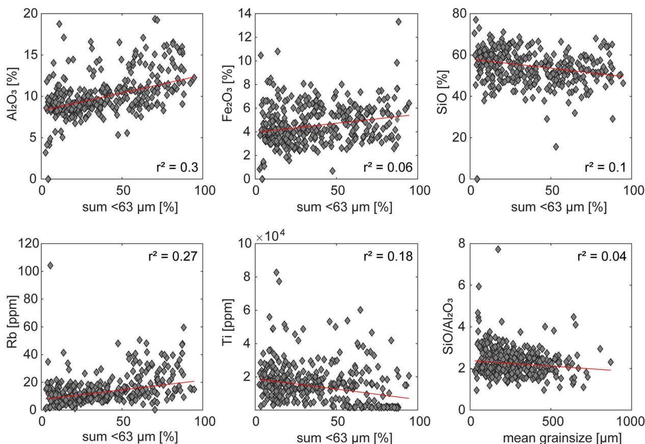
Fig. 4 The six plots depict the relation of the grain size, either given as sum of all grain size classes < 63 µm or as mean grain size, and common geochemical parameters used to approximate grain size characteristics. In addition, the coefficient of determination r^2 is given. For Al 2 O 3 , Fe 2 O 3 , Rb, and Ti, higher concentrations are expected in finer sediments, whereas the SiO content and the ratio of SiO to Al 2 O 3 , should decrease in finer sediments. Based on r^2 , the Al 2 O 3 content is the most suitable approximation of the fine material. Hence, Al was chosen as reference element for geochemical normalization
