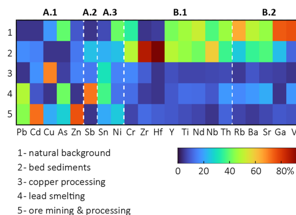
Fig. 14 Heatmap comparing the results obtained by investigating enrichment factors vs. PMF results. As denoted on the x-axis, the elements are sorted based on the grouping of elements as derived by EF ( A —anthropogenically influenced, B —dominated by natural processes). The rows indicate the five PMF factors, and the color scheme visualizes the amount of each element covered by the respective factor. It becomes apparent that the results are similar. However, PMF provides a somewhat deeper and more differentiated understanding
