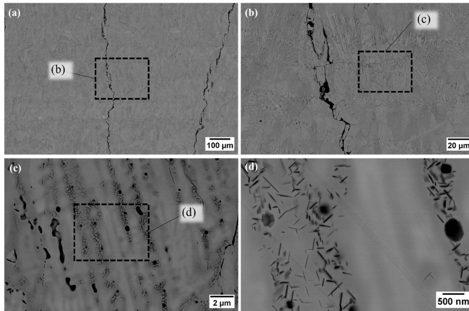
Fig. 7. SEM observation of RCCA#1 processed with HT-LPBF ( P=300 W, v=450 mm/s, h=75 \mu m). (a, b) Large cracks parallel to build direction. (c) Interdendritic segregation and shrinkage porosity. (d) Nanoprecipitates within interdendritic regions.
